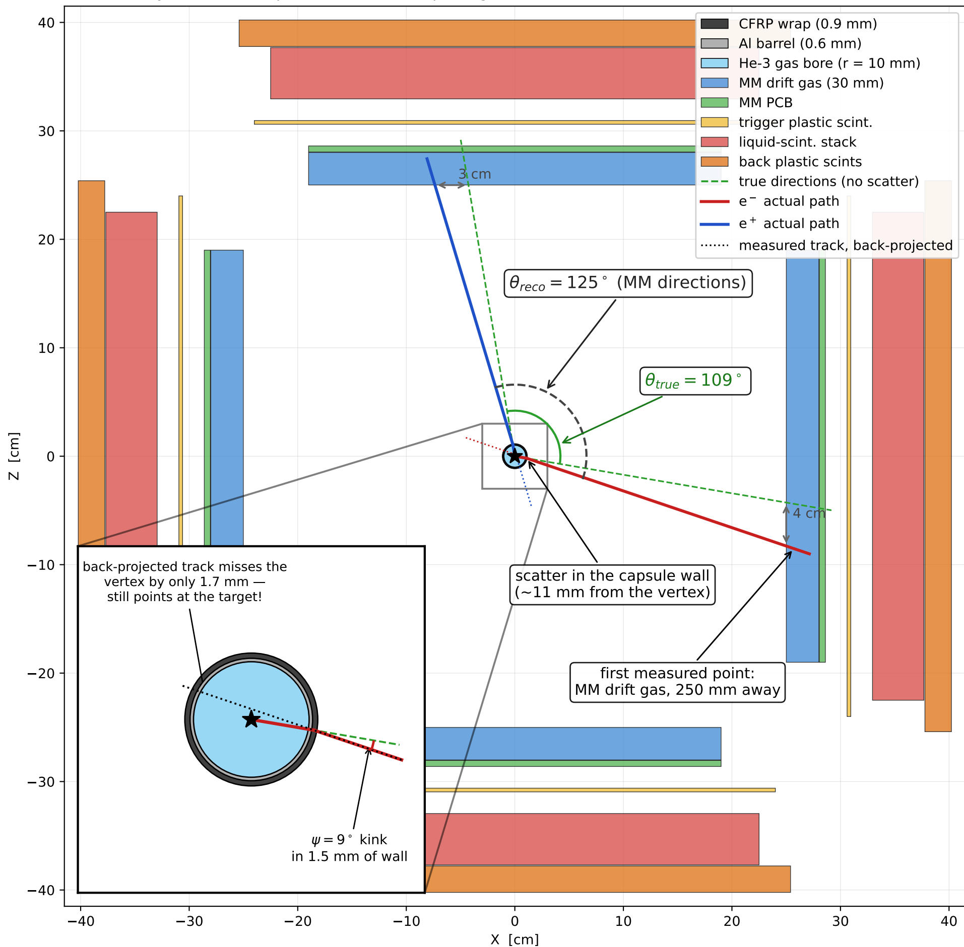
How the capsule wall destroys the opening angle — top-down view (beam into page) symmetric X17 pair, KE = 9.8 MeV per leg; wall kinks of 9^\circ/7^\circ ( \approx 1\sigma ) turn 109^\circ into 125^\circ
