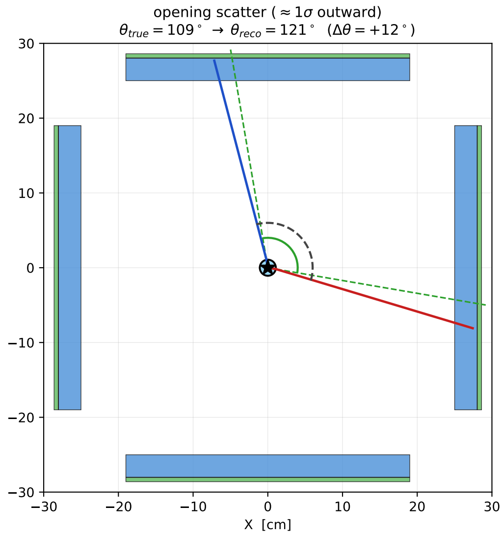
The same true pair, three throws of the scattering dice (per-leg \theta_0 \approx 7^\circ at KE = 9.8 MeV)
