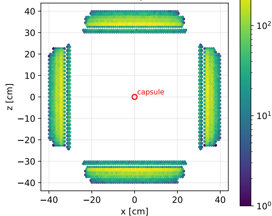
Capture positions, beam view (four-arm pattern)
