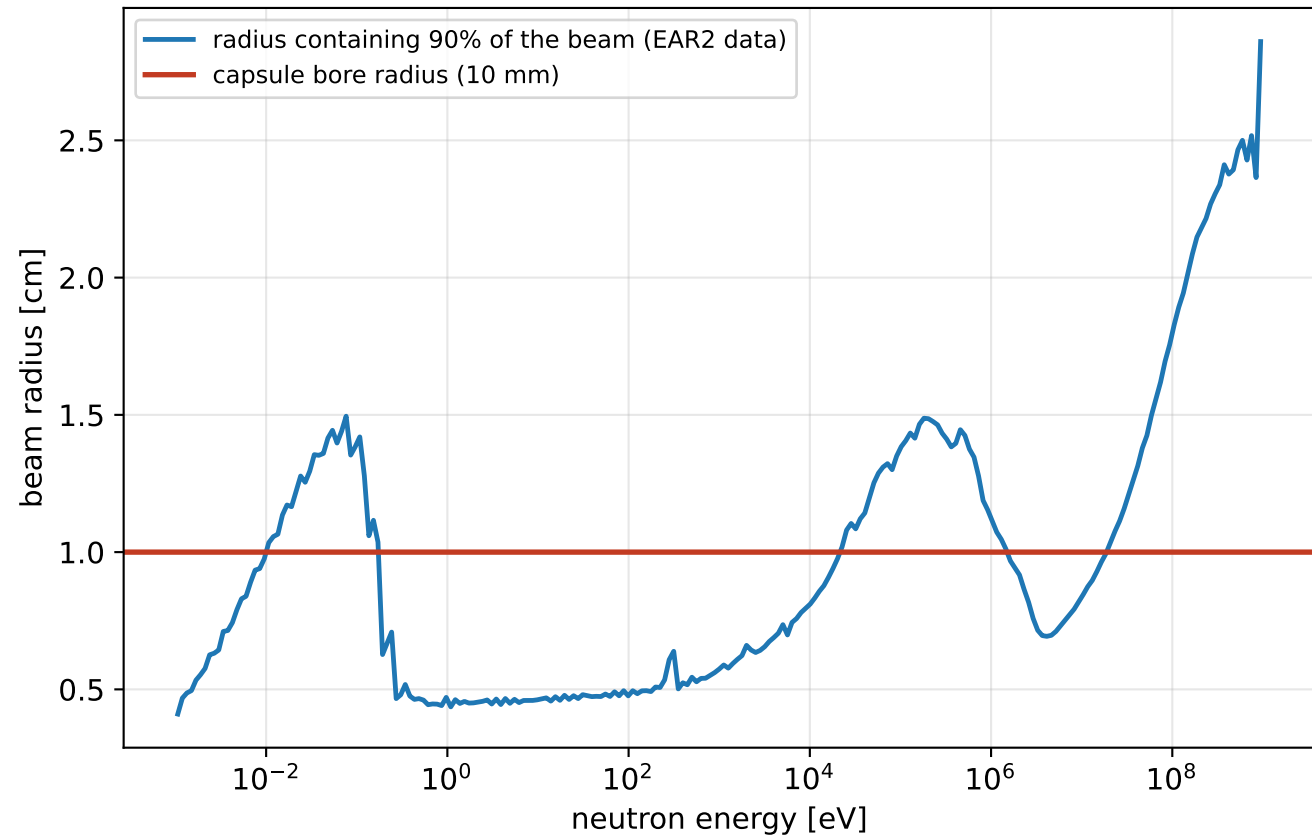
Beam footprint vs capsule bore: the halo misses the gas
