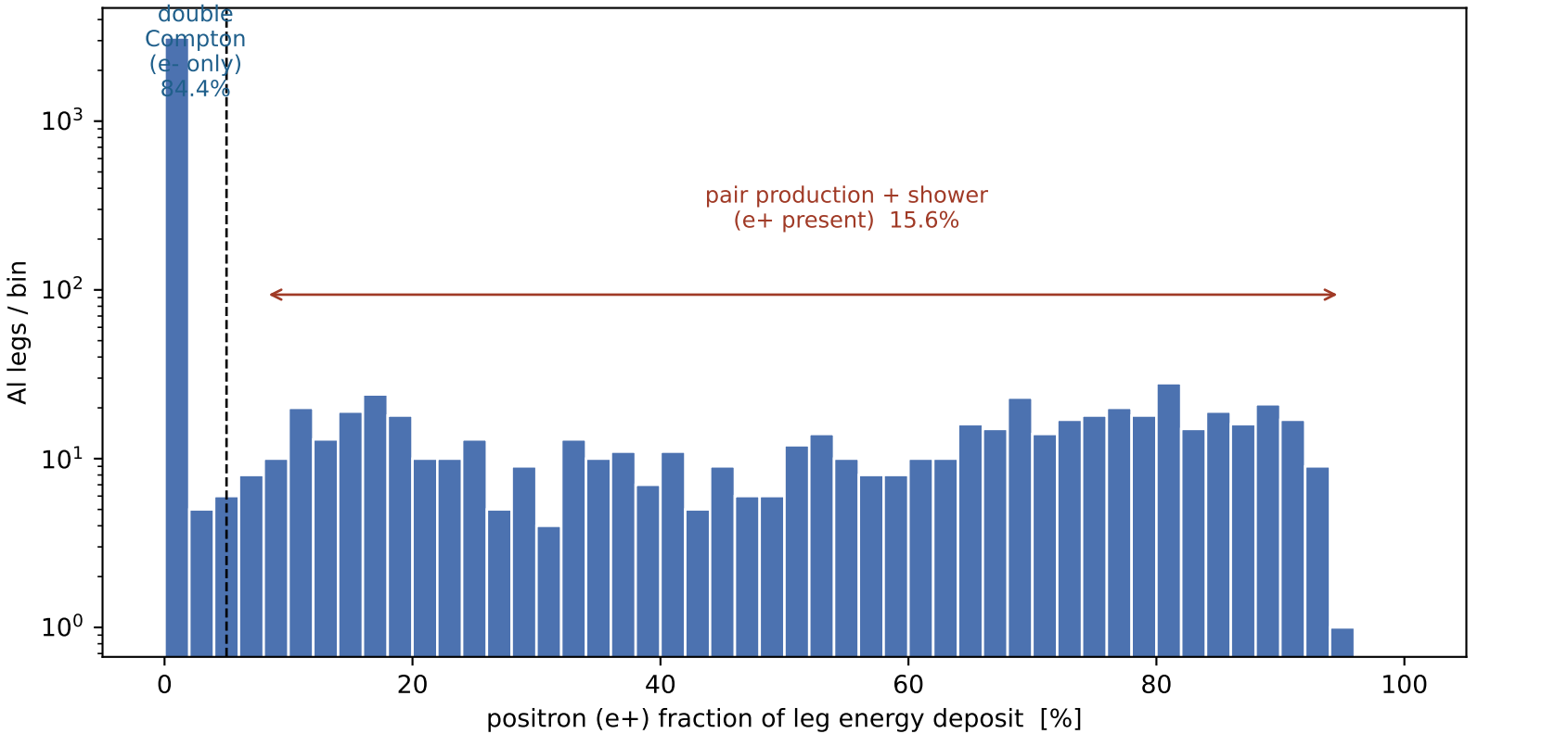
Al-capture leg mechanism: e+ energy fraction (N=3724; 84.4% double-Compton, 15.6% pair-production)
