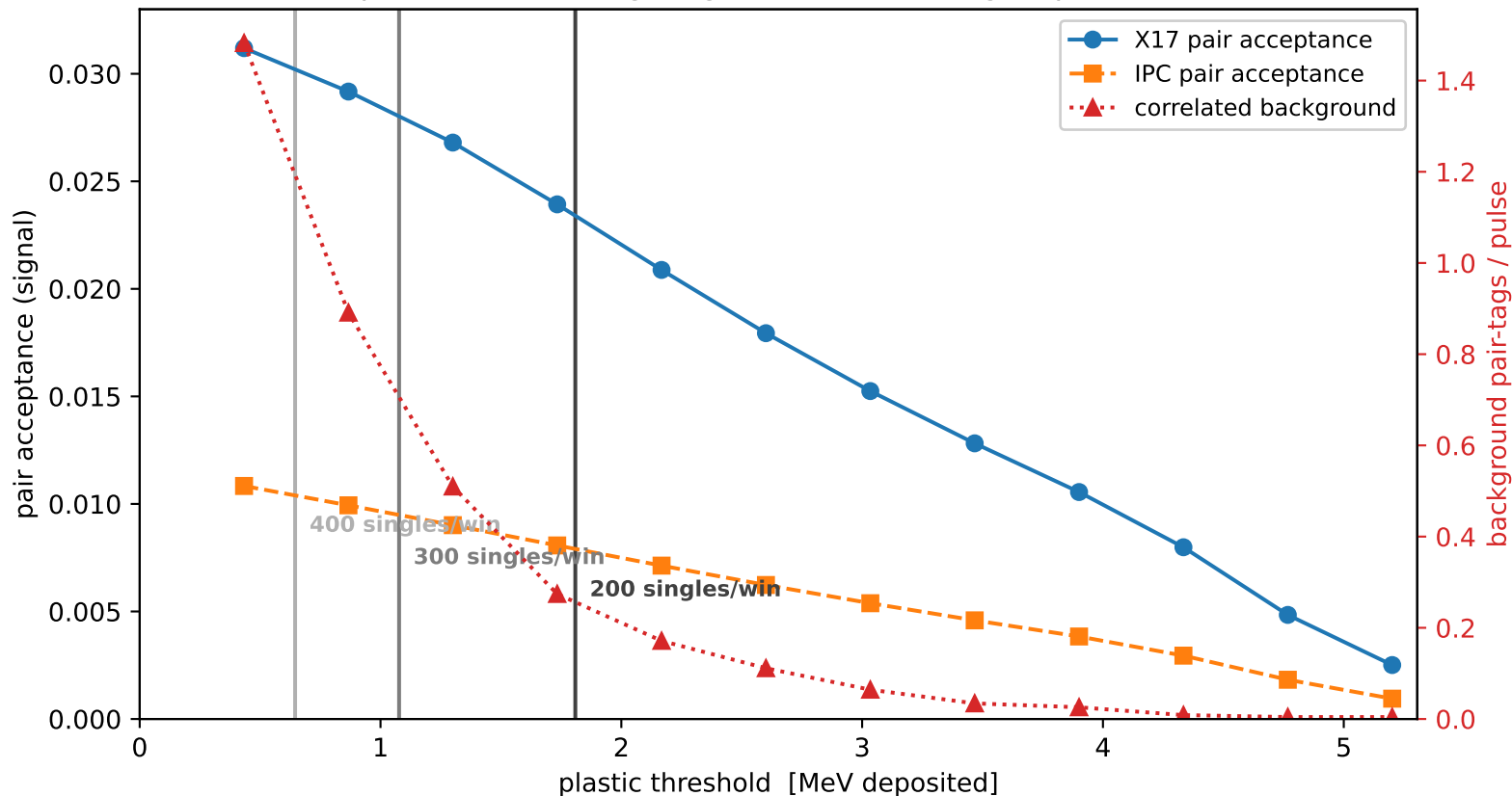
Signal & background vs plastic threshold (SiPM 0.5 MIP) vertical lines = plastic threshold giving 200/300/400 singles per window (OR of walls)
