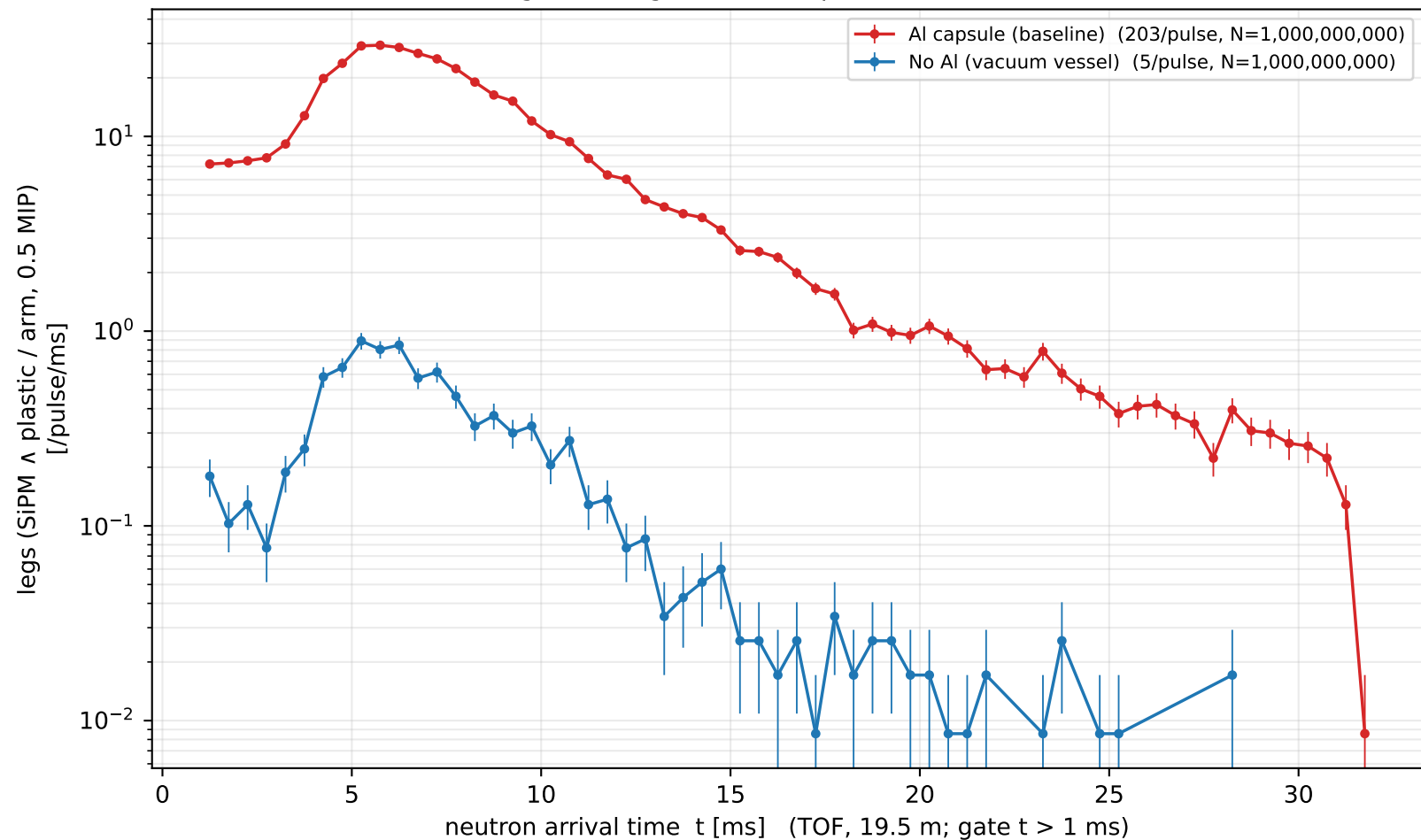
Thermal-gate background: Al capsule vs. no-Al cross-check
