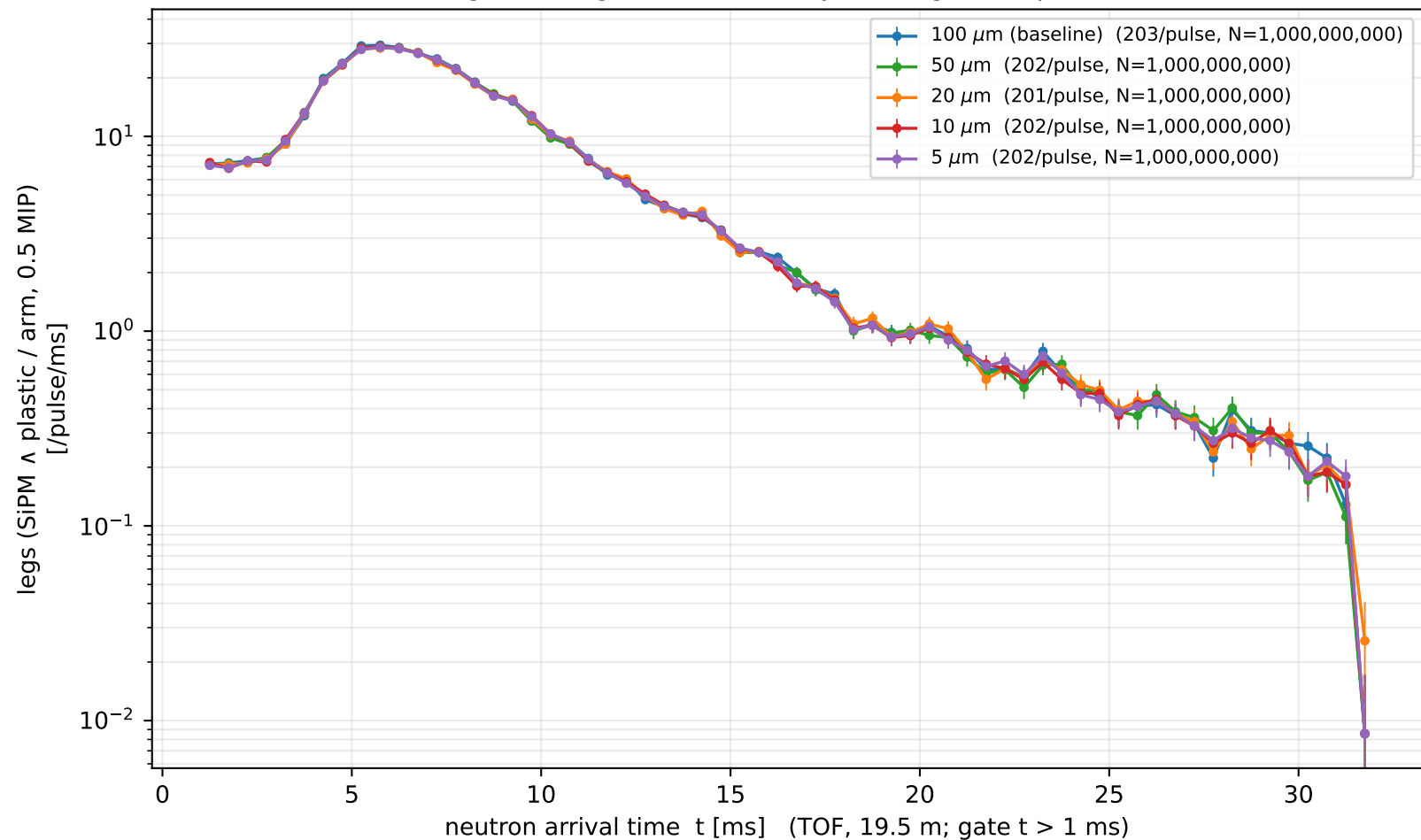
Thermal-gate background: sensitivity to the gamma production cut
