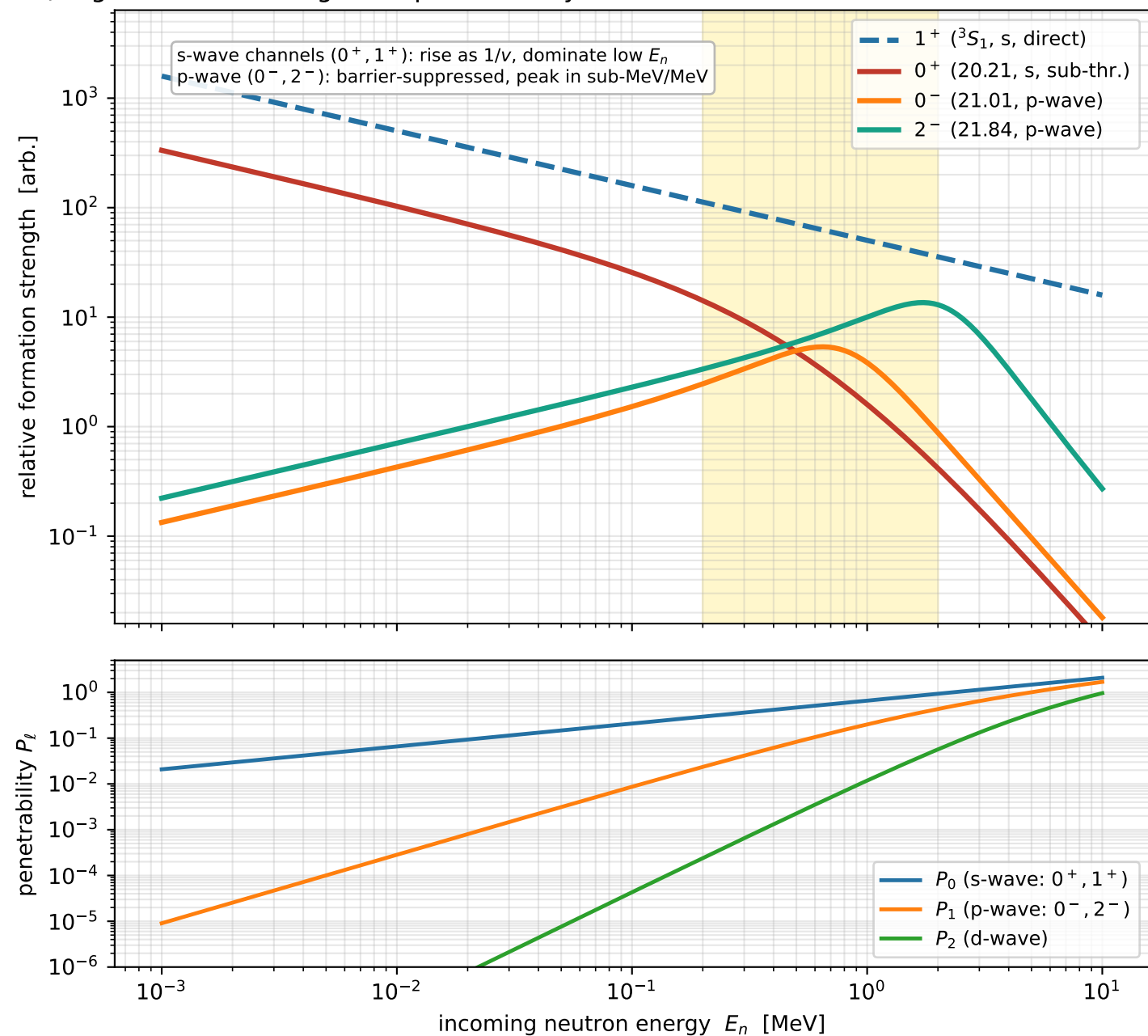
Which {}^4\text{He}^* doorway do we form, vs neutron energy? (single-level Breit-Wigner \times penetrability; TUNL A=4, a = 4 fm. 1^+ is direct/non-resonant.)
