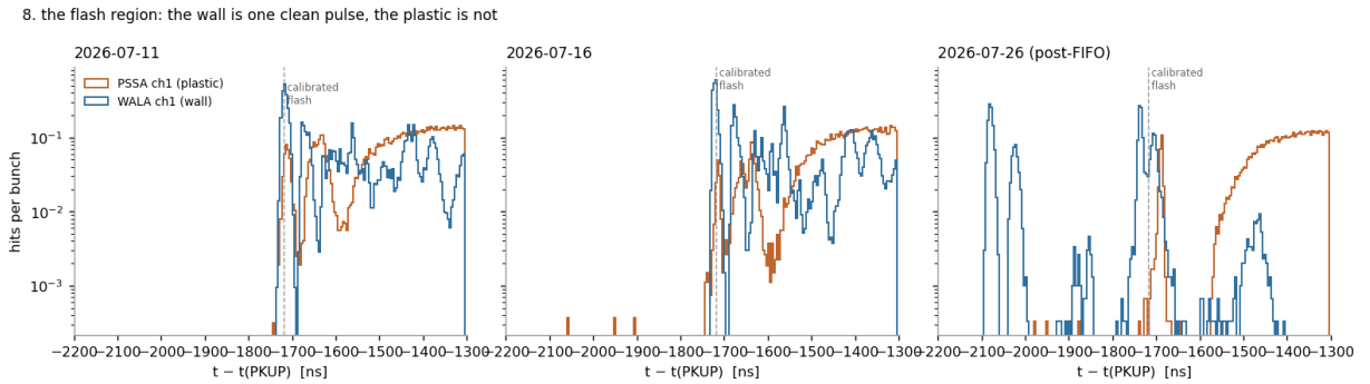
Figure 7: Hit density per bunch in the flash region. The wall produces one clean pulse; the plastic response is spread over \sim 100 ns and accompanied by a continuum of fragments. In the post-FIFO run the wall shows both the gate transient ( \sim -2100 ns) and the leak ( \sim -1750 ns).
