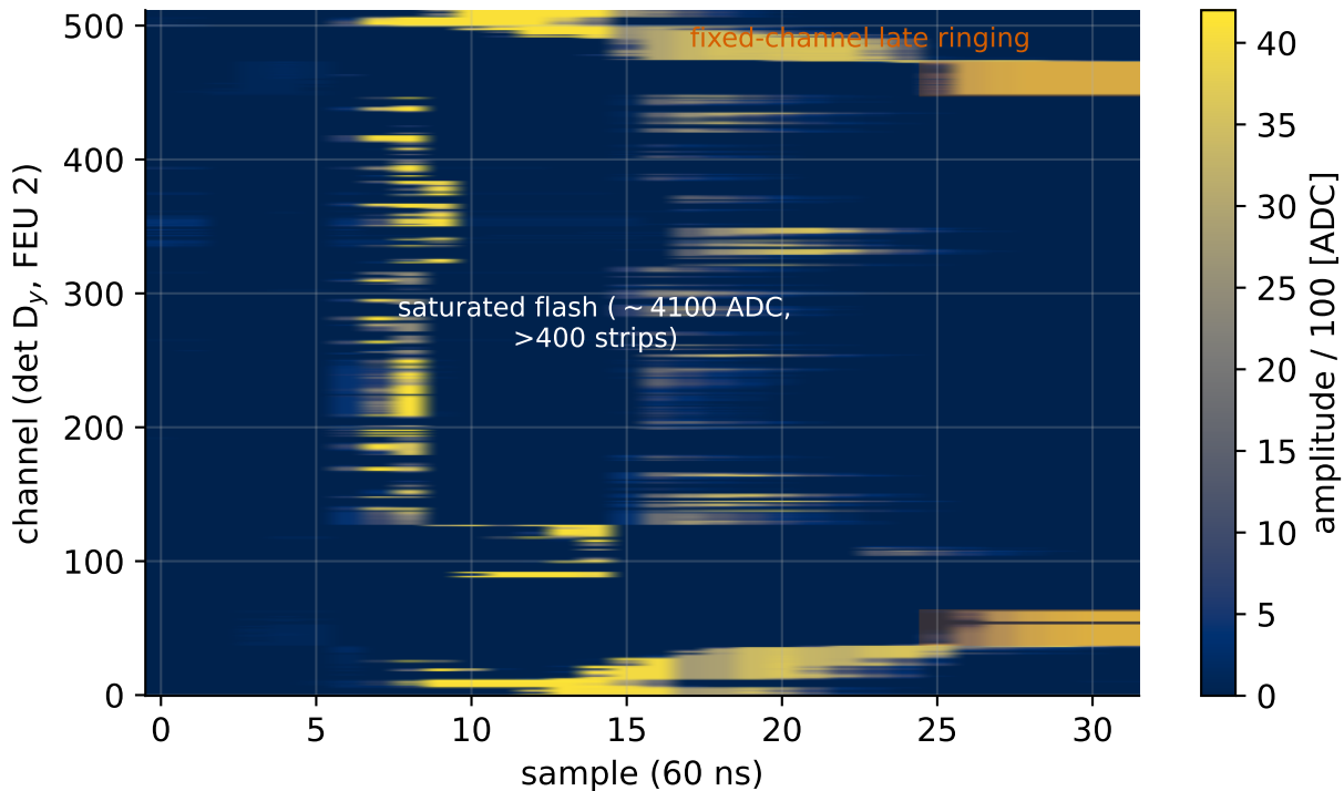
beam flash/"monster" event (run_55): the source of fake late edges
