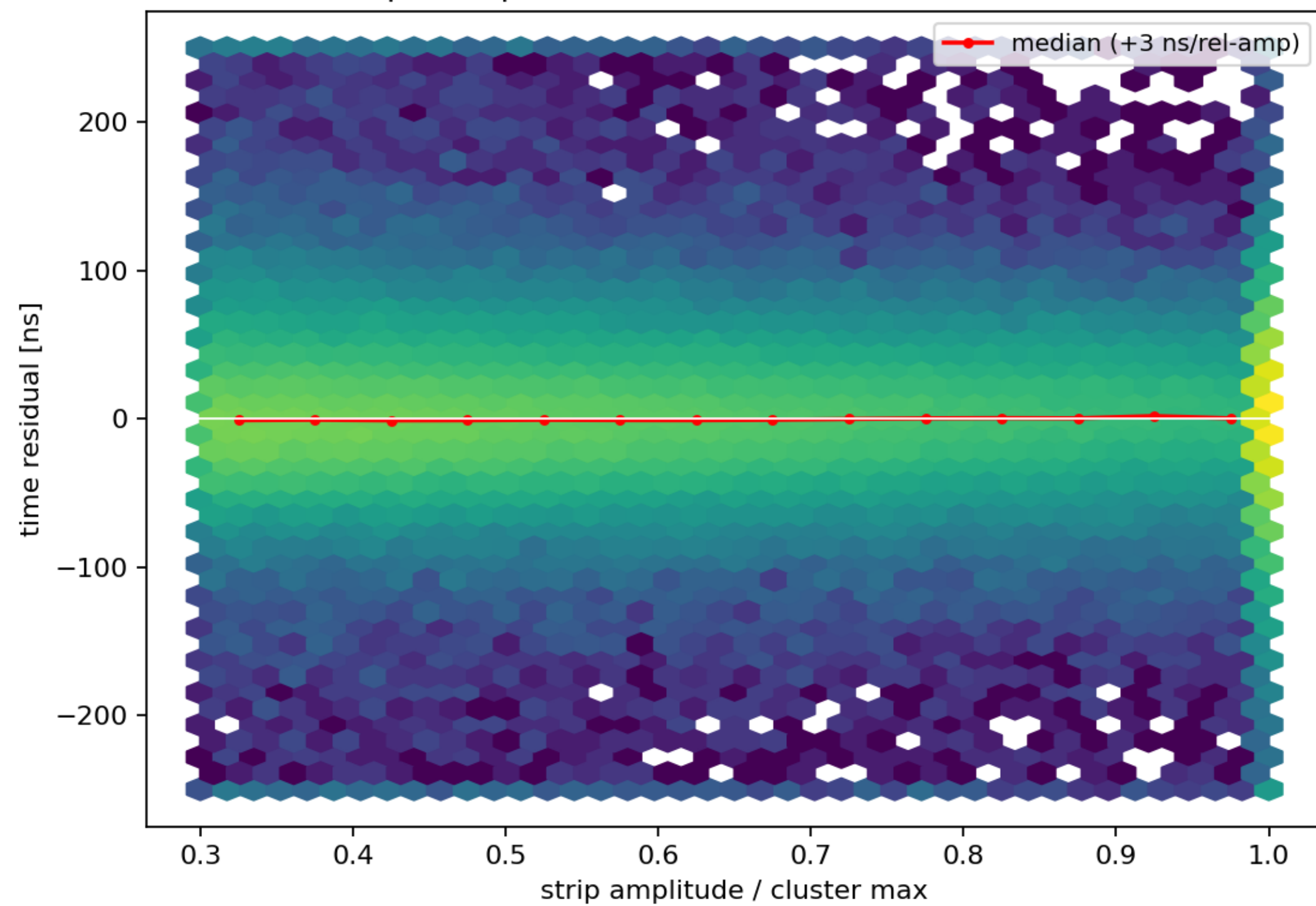
per-strip time-walk (correctable calibration)
