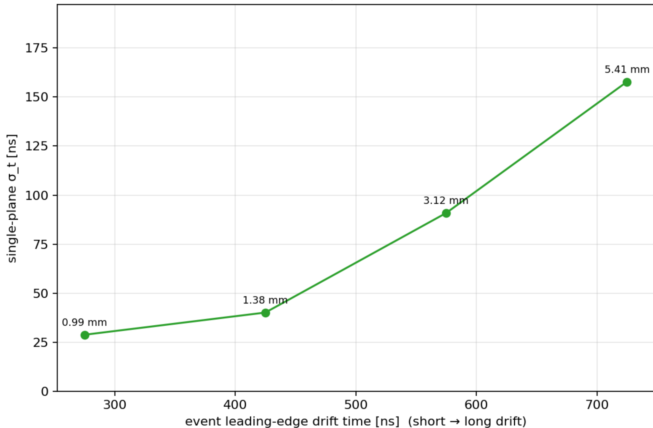
time resolution vs drift depth (diffusion + attachment S/N)
