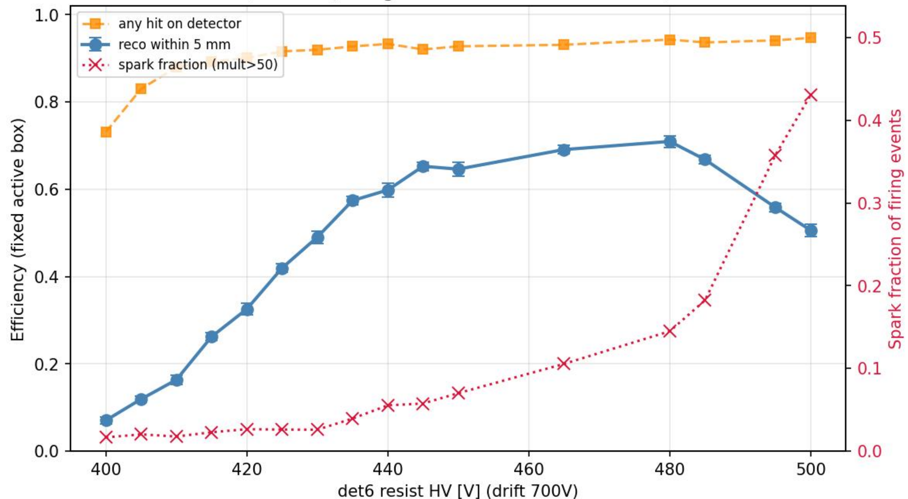
mx17_6 efficiency + spark rate vs hv_scan — mx17_det6_det7_hv_scan_6-26-26 ( r < 5 mm; integrated over fixed active area)
