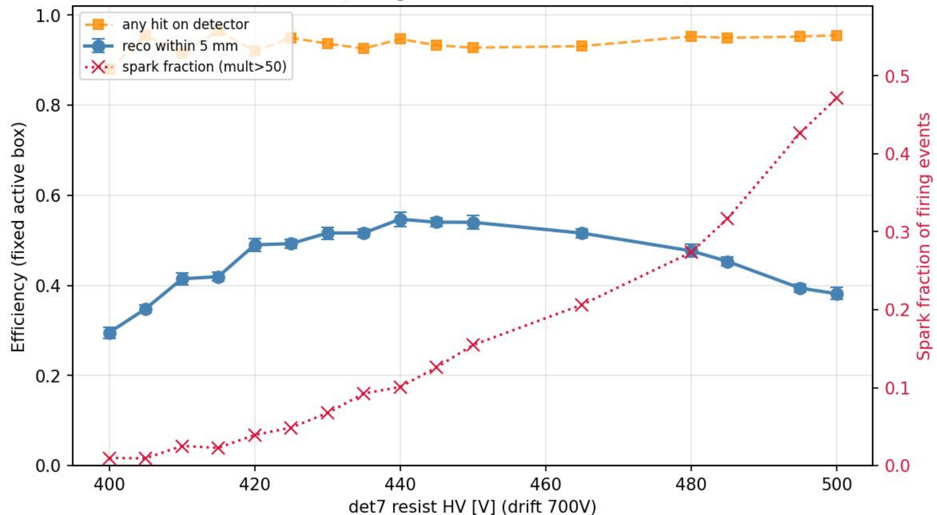
mx17_7 efficiency + spark rate vs hv_scan — mx17_det6_det7_hv_scan_6-26-26 ( r < 5 mm; integrated over fixed active area)
