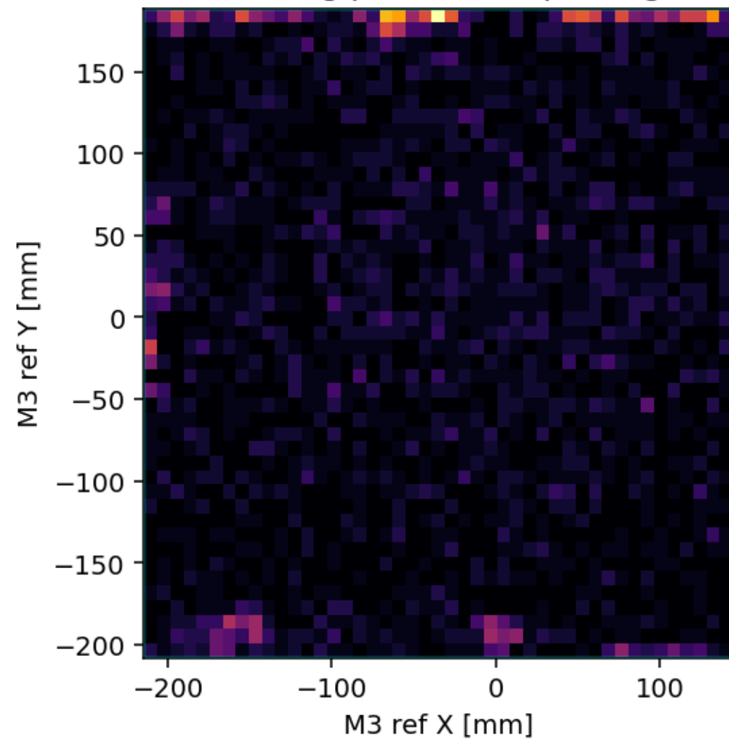
(b) M3 crossing position of sparking muons
