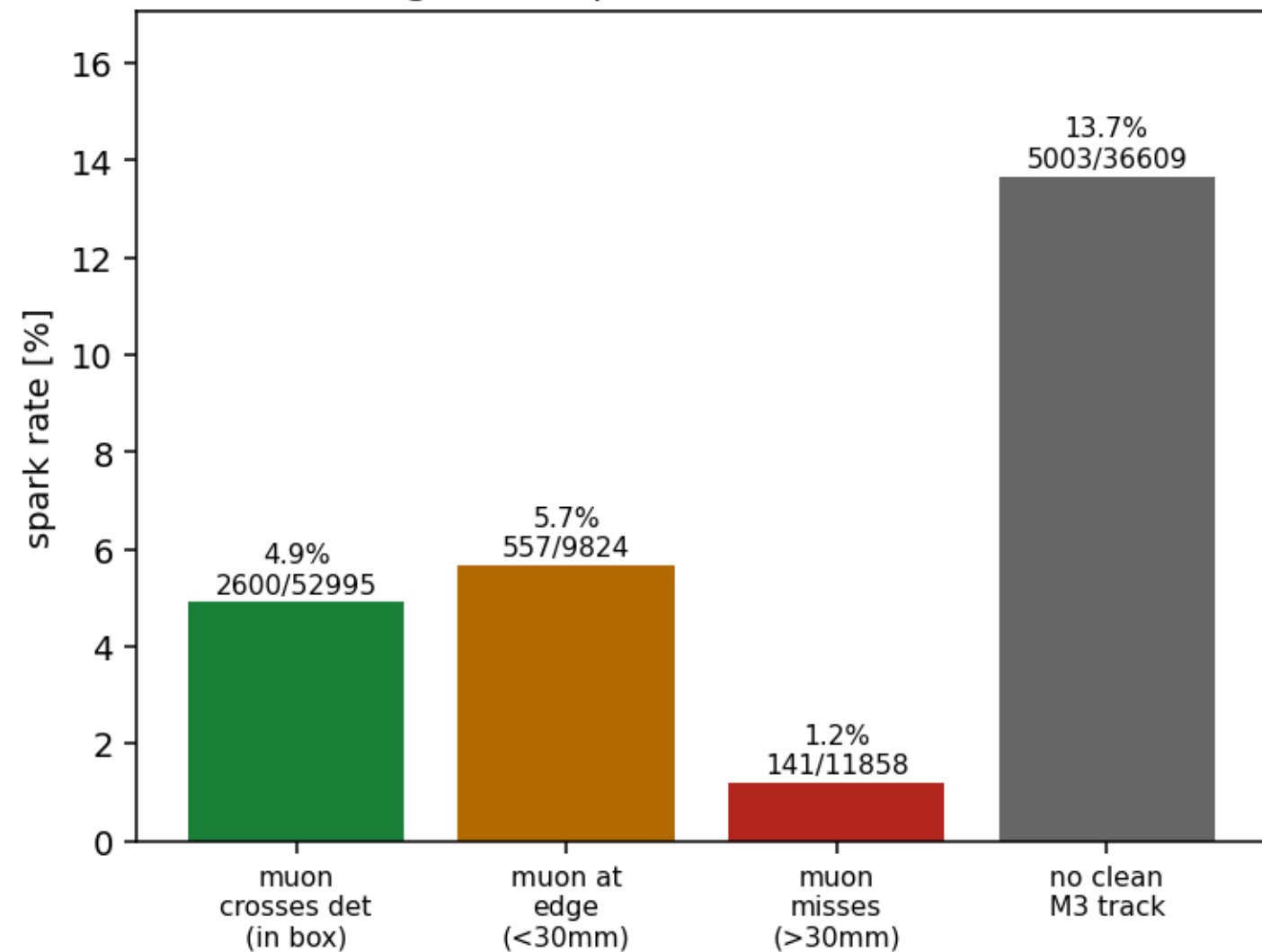
(a) spark rate vs muon geometry crossing muon sparks 4x more than a miss
