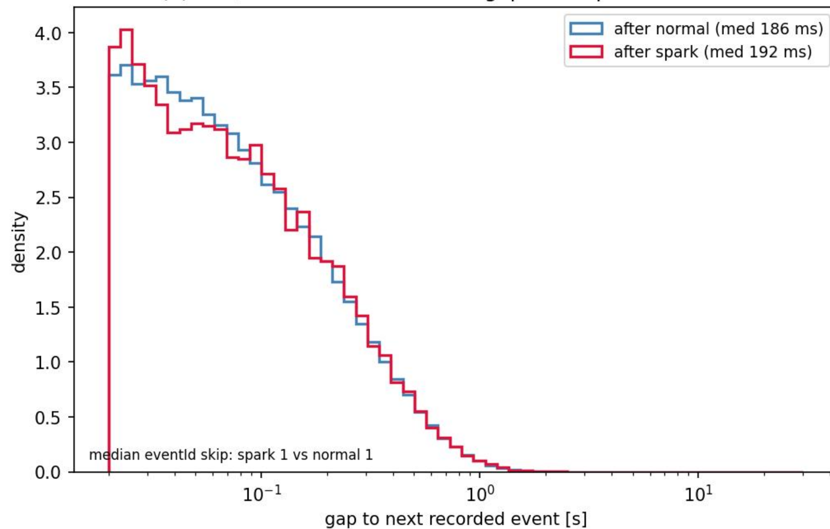
(a) DAQ dead time: next-event gap after spark vs normal
