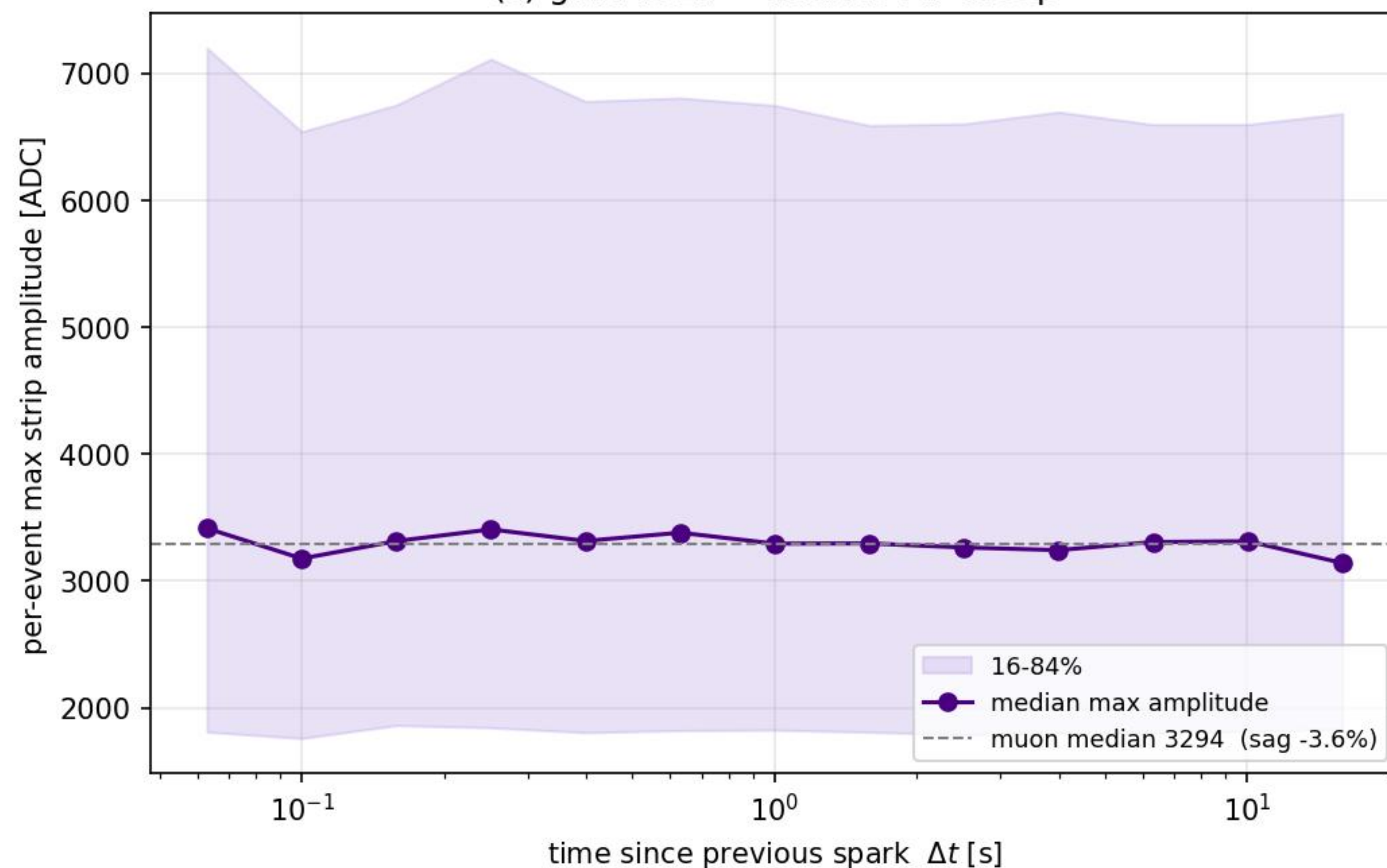
(c) gain vs \Delta t — flat: no HV droop
