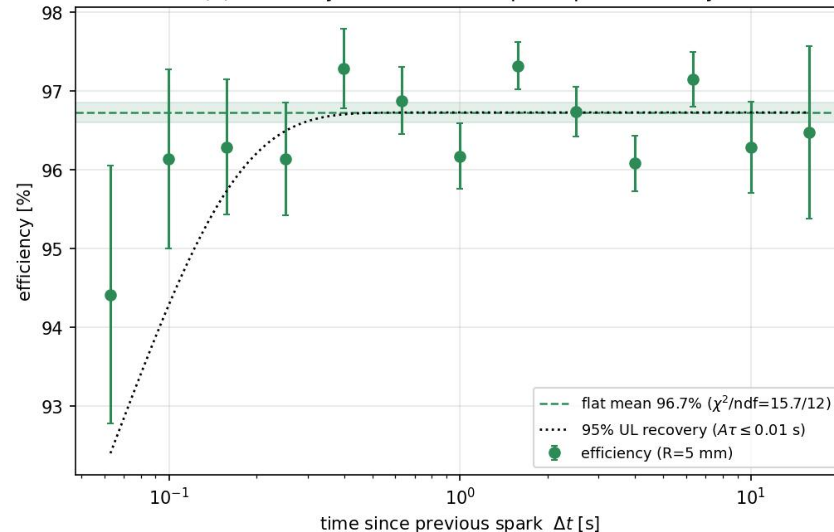
(b) efficiency vs \Delta t — flat: no post-spark recovery
