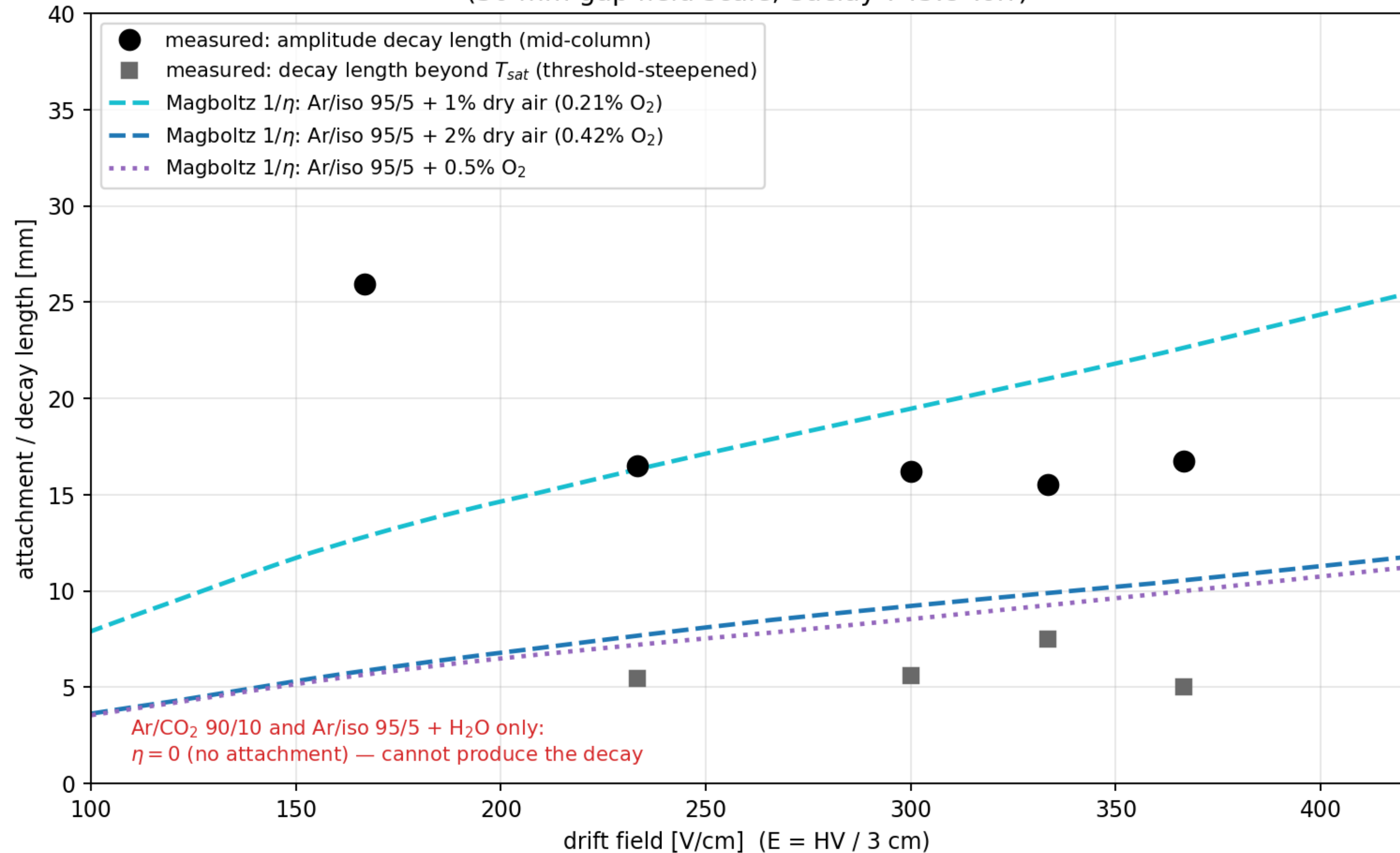
mx17_3 measured signal-decay length vs Magboltz attachment (30 mm gap field scale, Saclay 745.8 Torr)
