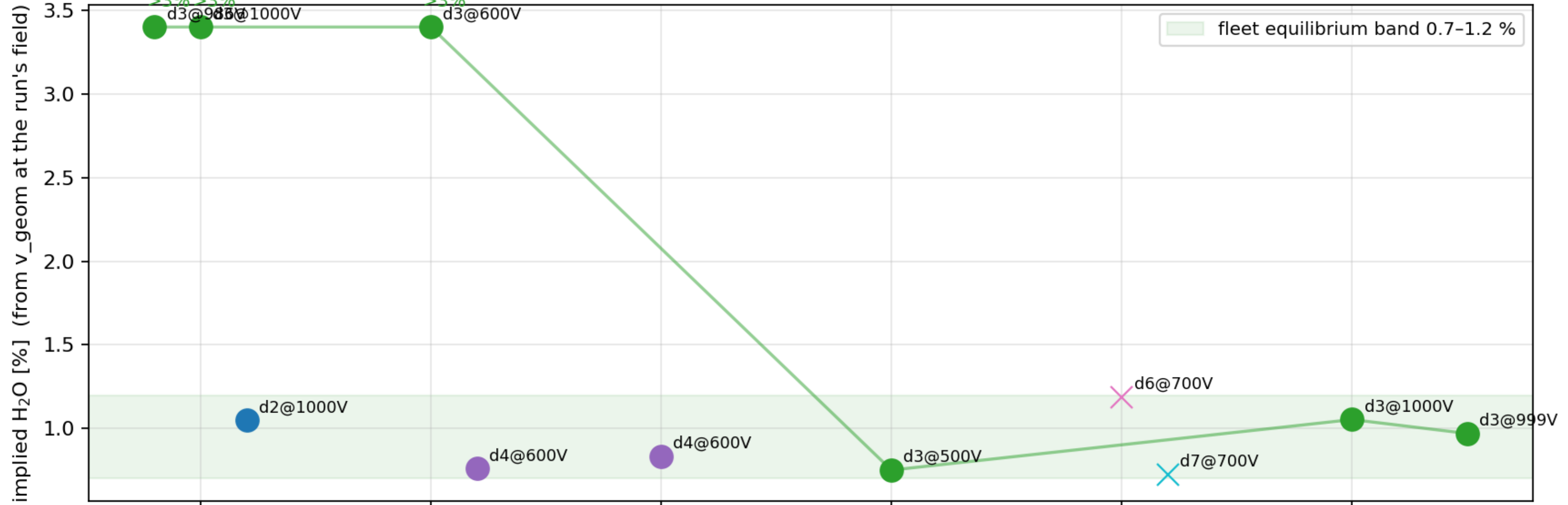
water content vs date — det3 dries from >3 % to ~1 %
