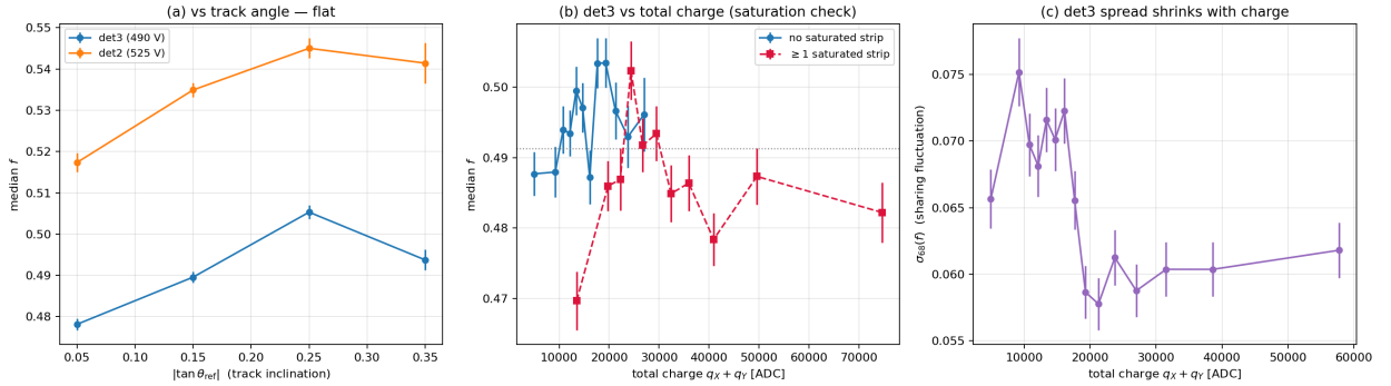
Figure 6: (a) median f vs track angle — flat for both chambers. (b) det3 f vs total charge, split by saturated-strip presence: the saturation correction leaves f unbiased to the quoted systematic. (c) the sharing fluctuation \sigma_{68}(f) decreases with signal size.
