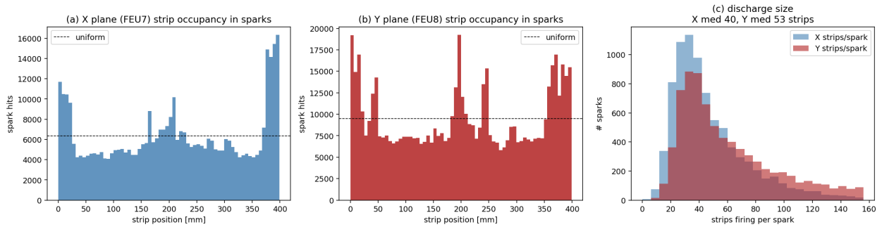
Figure 3: Where. (a,b) strip occupancy in sparks for the X and Y planes vs a uniform baseline — edge peaks (both planes) and fixed hot strips ( Y ); (c) strips firing per spark — Y discharges are larger than X .
