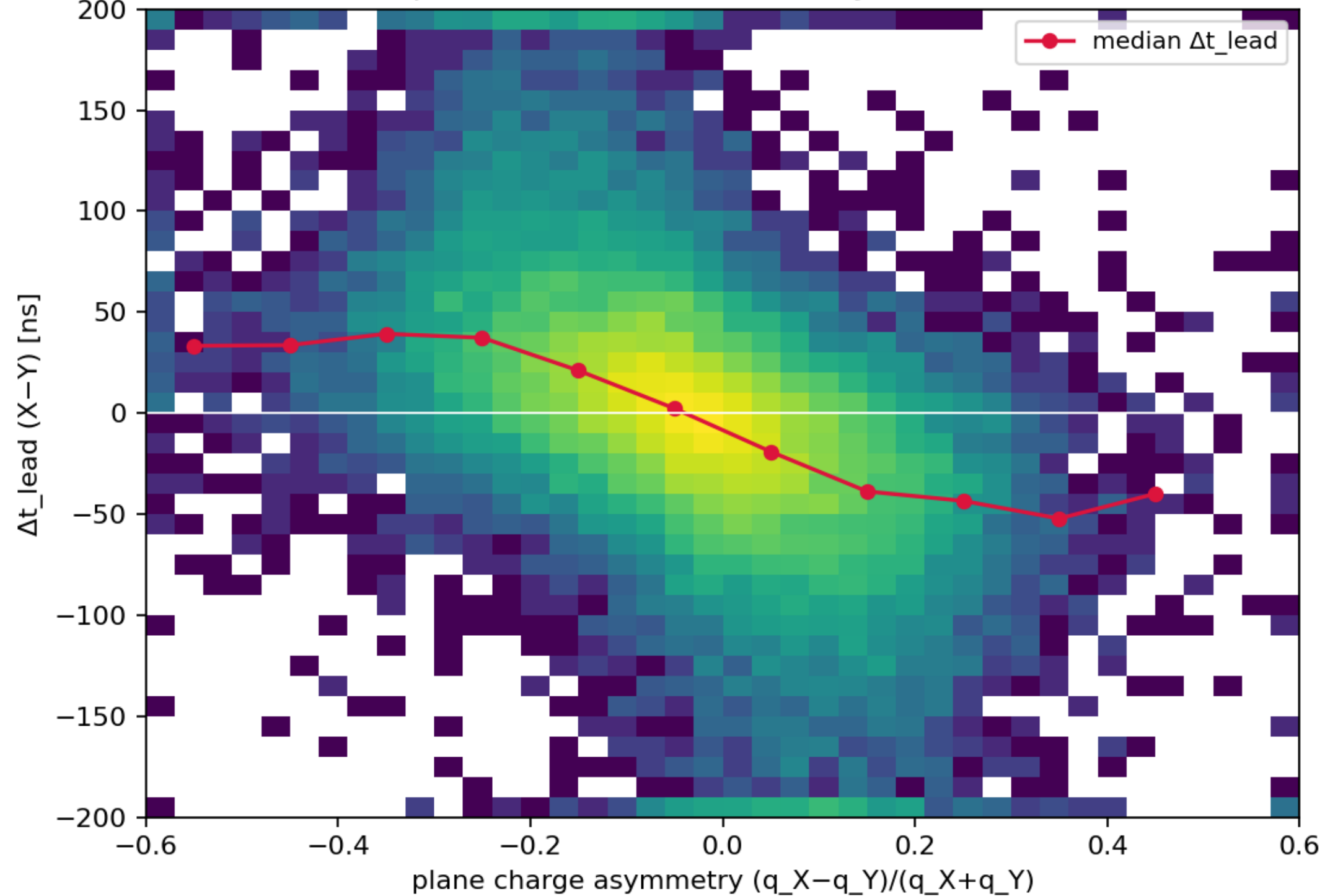
inter-plane time-walk (-105 ns/asym \rightarrow 33 \rightarrow 29 ns)
