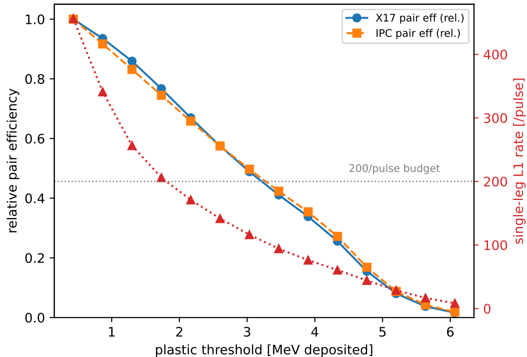
Full 2-leg coincidence (SiPM 0.5 MIP fixed)
