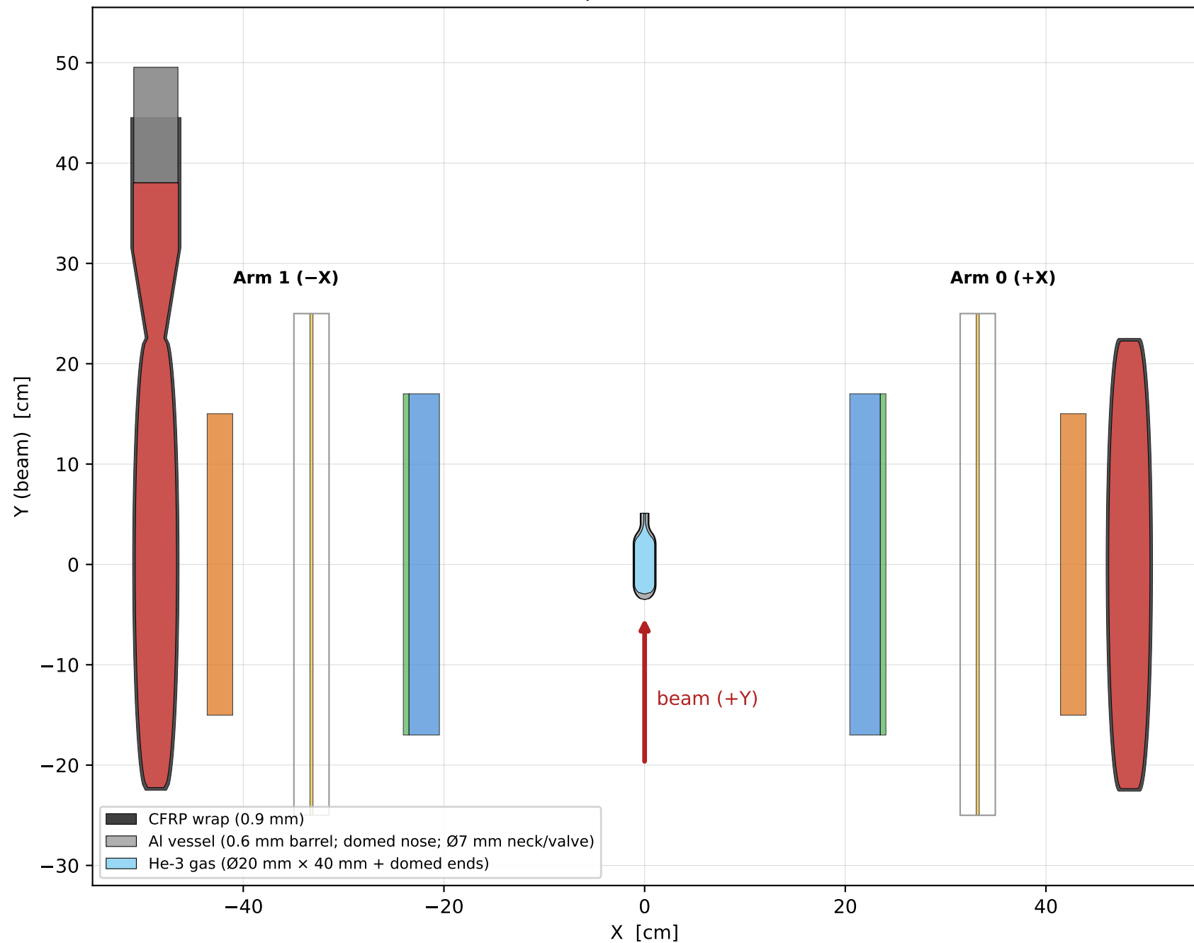
MX17 Geometry — Side View (XY plane) Beam from below hits the capsule end-on; arms 2,3 ( \pm Z ) not shown
