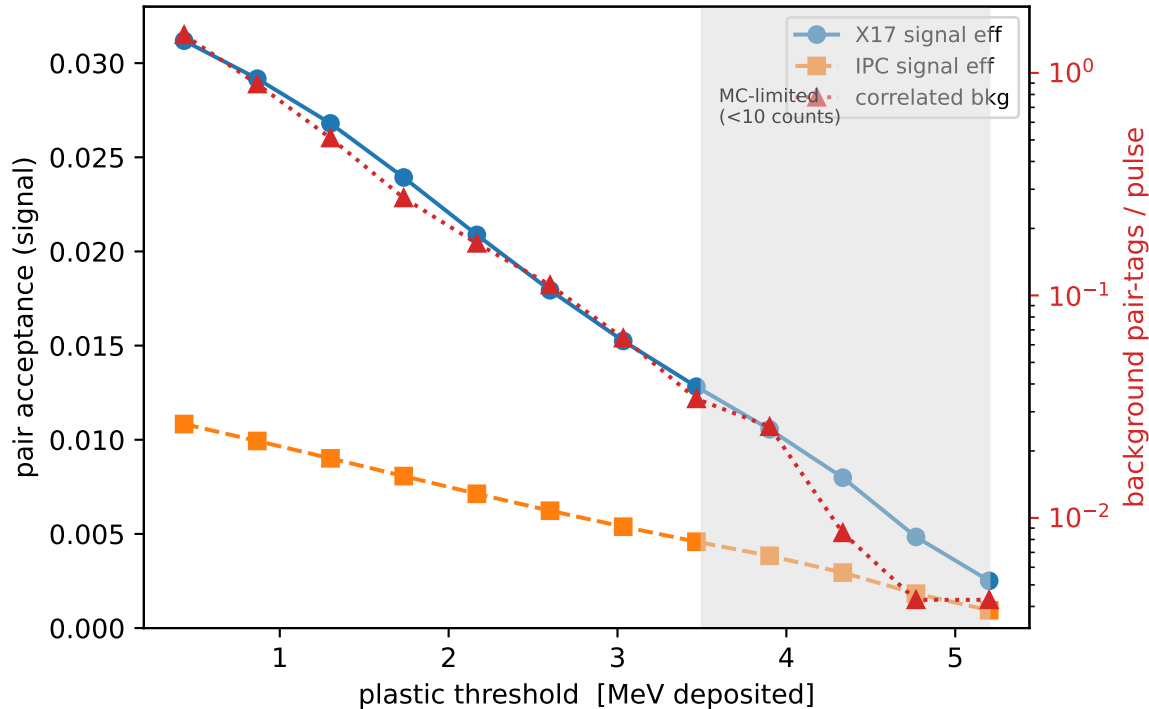
Signal vs correlated background (SiPM 0.5 MIP)
