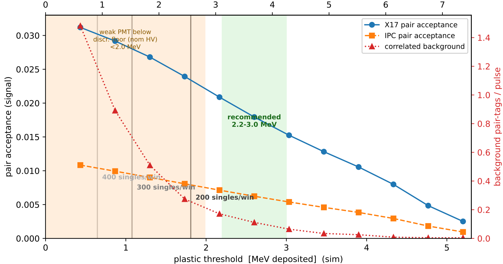
Signal & background vs plastic threshold (SiPM 0.5 MIP) MeV->mV via beam MIP calib (run224489); vertical lines = sim singles/window plastic threshold [mV, median PMT @ nominal HV] (1 MIP = 6.1 mV)
