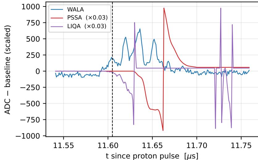
the same flash in three detectors, 11.60 \mu s
