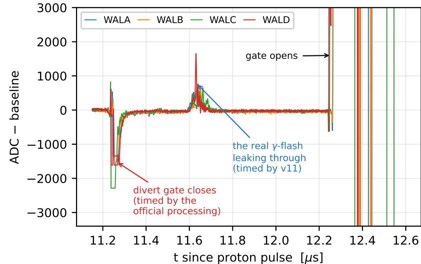
SiPM wall: what the divert leaves behind
