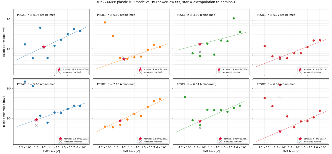
Figure 14: Plastic MIP mode vs. HV with the coincident-median power law anchored to the trusted ( V \geq 1400 V) modes; the star is the nominal-HV MIP, the gray cross the (threshold-biased) directly measured nominal mode.
