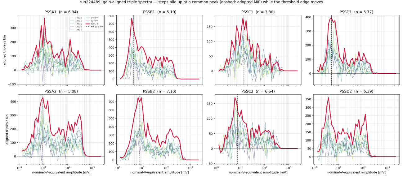
Figure 11: Gain-aligned triple-tagged plastic spectra: thin curves are individual steps ( V \geq 1300 V) scaled to nominal-V equivalent, the red curve is their sum ( /3 ), the dashed line the adopted MIP. A physical peak aligns; the threshold edge does not.
