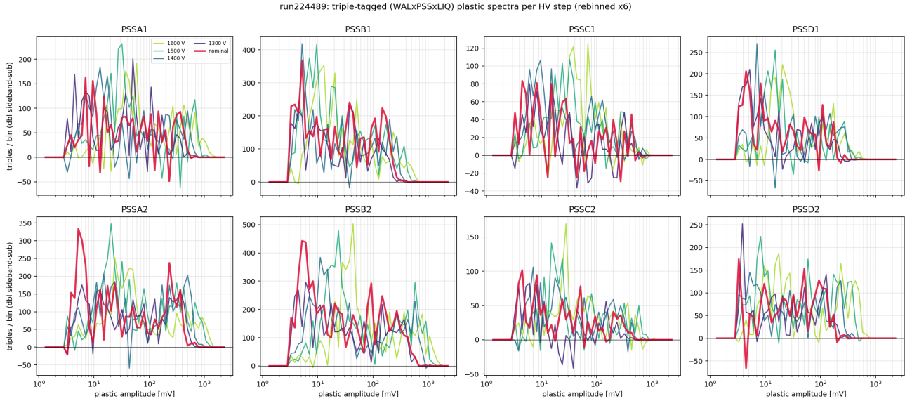
Figure 12: Triple-tagged plastic spectra per HV step (double sideband-subtracted, rebinned \times 6 ; readable subset of steps shown). The MIP hump moves coherently with HV; the red curve is the nominal-HV window.
