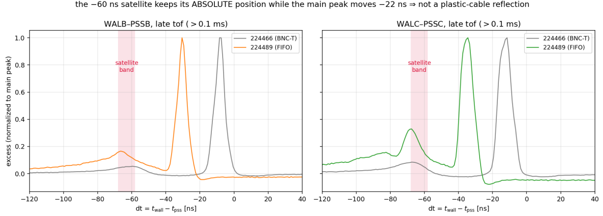
Figure 18: Late-tof dt spectra, normalized to the main peak, both runs.
