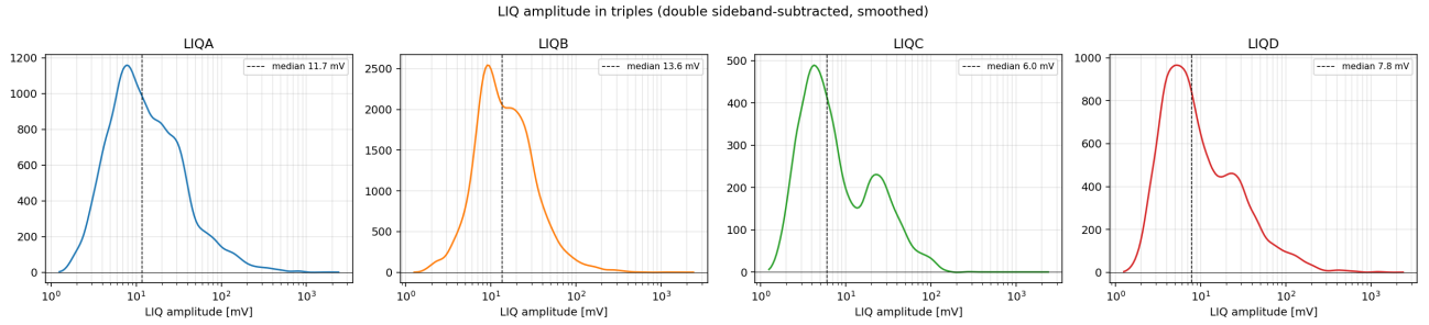
Figure 16: Triple-tagged LIQ amplitude spectra per arm.
