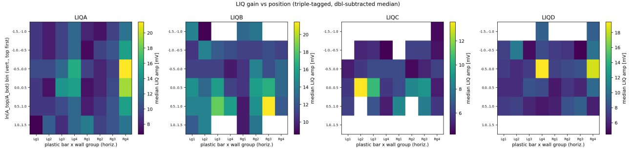
Figure 14: Median LIQ amplitude per position bin (triple-tagged, double sideband-subtracted). Columns: plastic bar \times wall group (left→right as seen from the back); rows: vertical asymmetry bins (negative = hit near the bottom).
