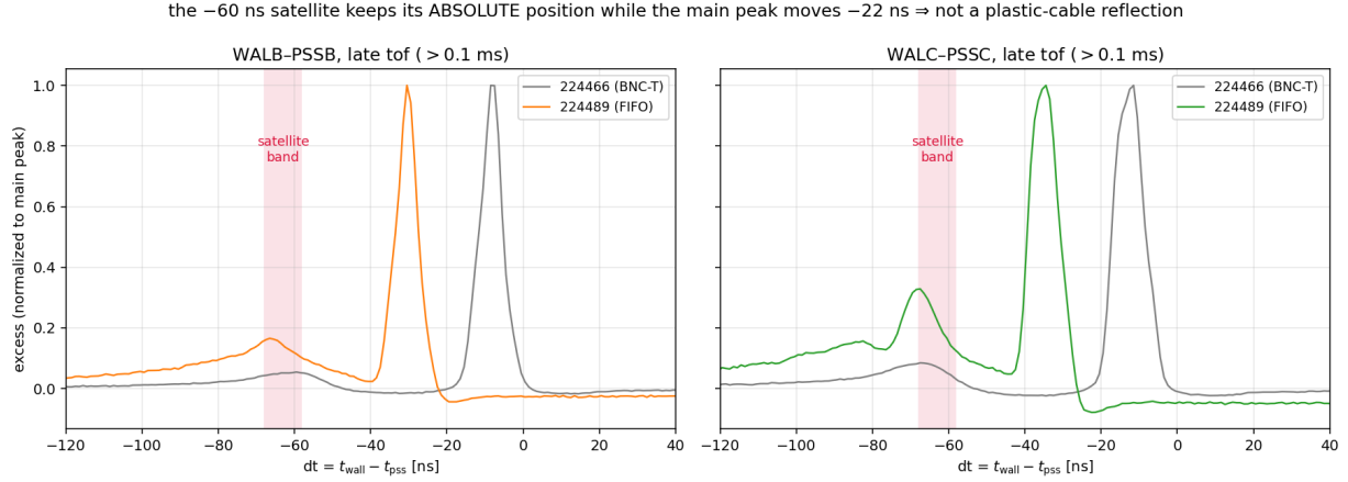
Figure 17: Late-tof dt spectra, normalized to the main peak, both runs.
