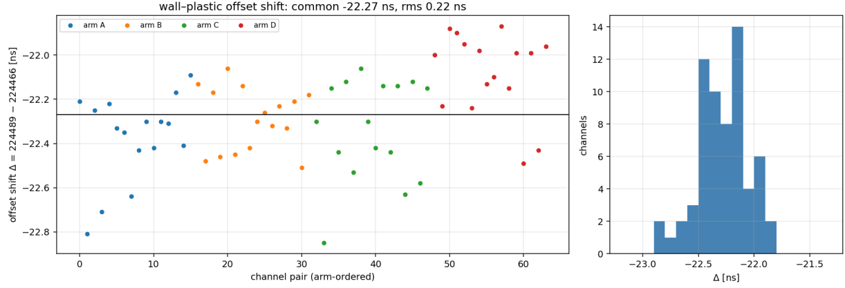
Figure 16: Per-channel offset shift between runs.
