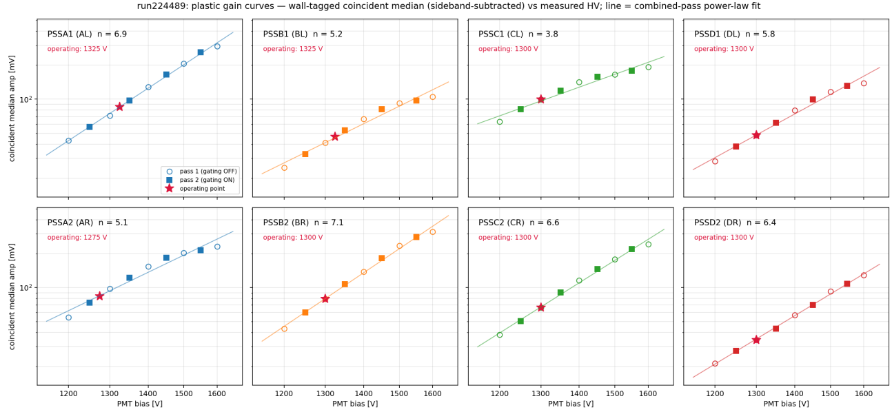
Figure 4: Coincident-median gain curves per PMT with power-law fits; the red star marks the operating point in the post-scan window.
