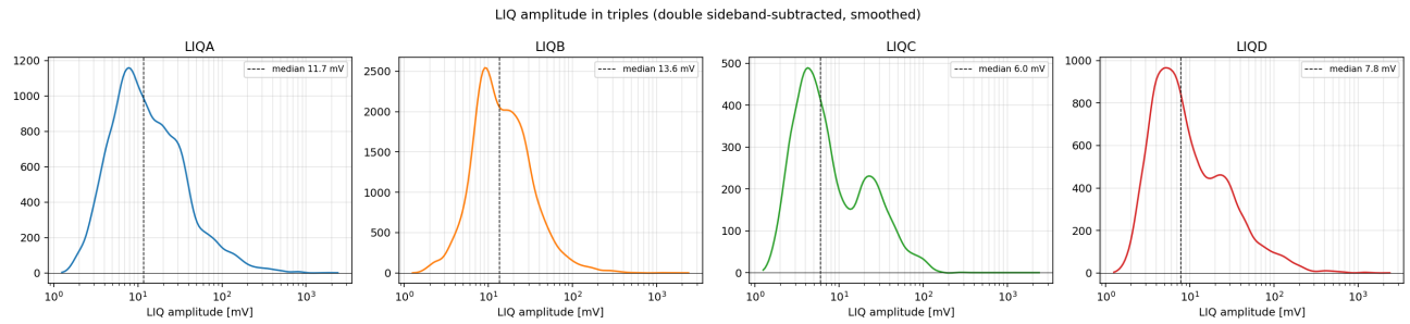
Figure 15: Triple-tagged LIQ amplitude spectra per arm.
