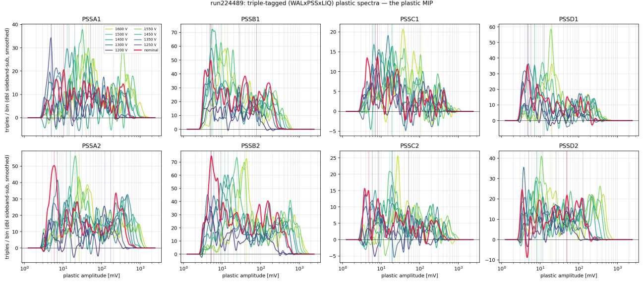
Figure 11: Triple-tagged plastic spectra per HV step (double sideband-subtracted, smoothed). The MIP hump moves coherently with HV; the red curve is the nominal-HV window.
