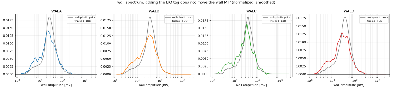
Figure 12: Wall spectra in wall-plastic pairs vs. triples (normalized): the LIQ tag does not move the wall MIP.
