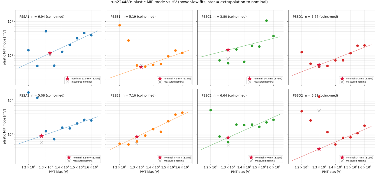
Figure 13: Plastic MIP mode vs. HV with the coincident-median power law anchored to the trusted ( V \geq 1400 V) modes; the star is the nominal-HV MIP, the gray cross the (threshold-biased) directly measured nominal mode.
