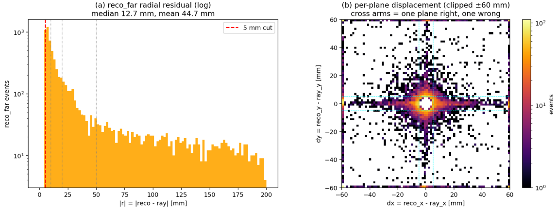
Figure 3: Residual structure. (a) reco_far radial residual (log y ): smooth fall-off plus a flat far plateau. (b) per-plane displacement ( dx, dy ), clipped \pm 60 mm; cyan lines mark \pm 5 mm. The cross arms are one-plane-wrong events; the diffuse cloud is both-planes-wrong.
