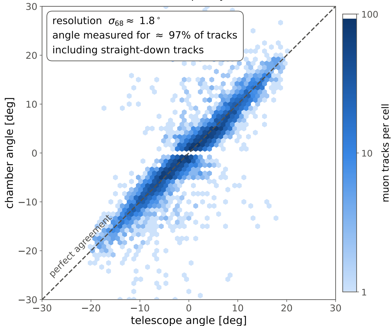
Track angle from the chamber alone vs reference telescope (hybrid method)
