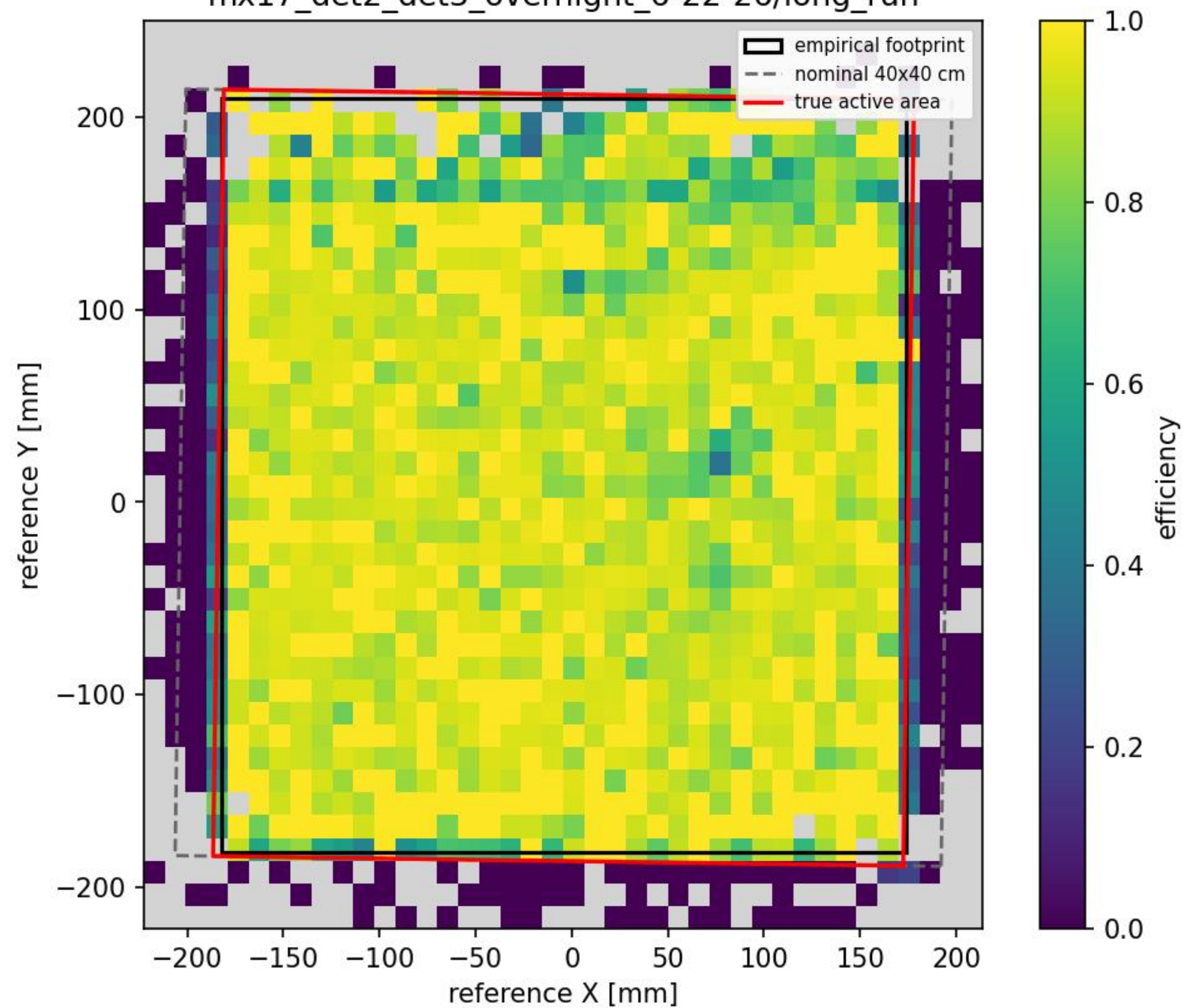
mx17_2 efficiency map — hit within 5 mm ( \geq 5 rays/bin) mx17_det2_det3_overnight_6-22-26/long_run
