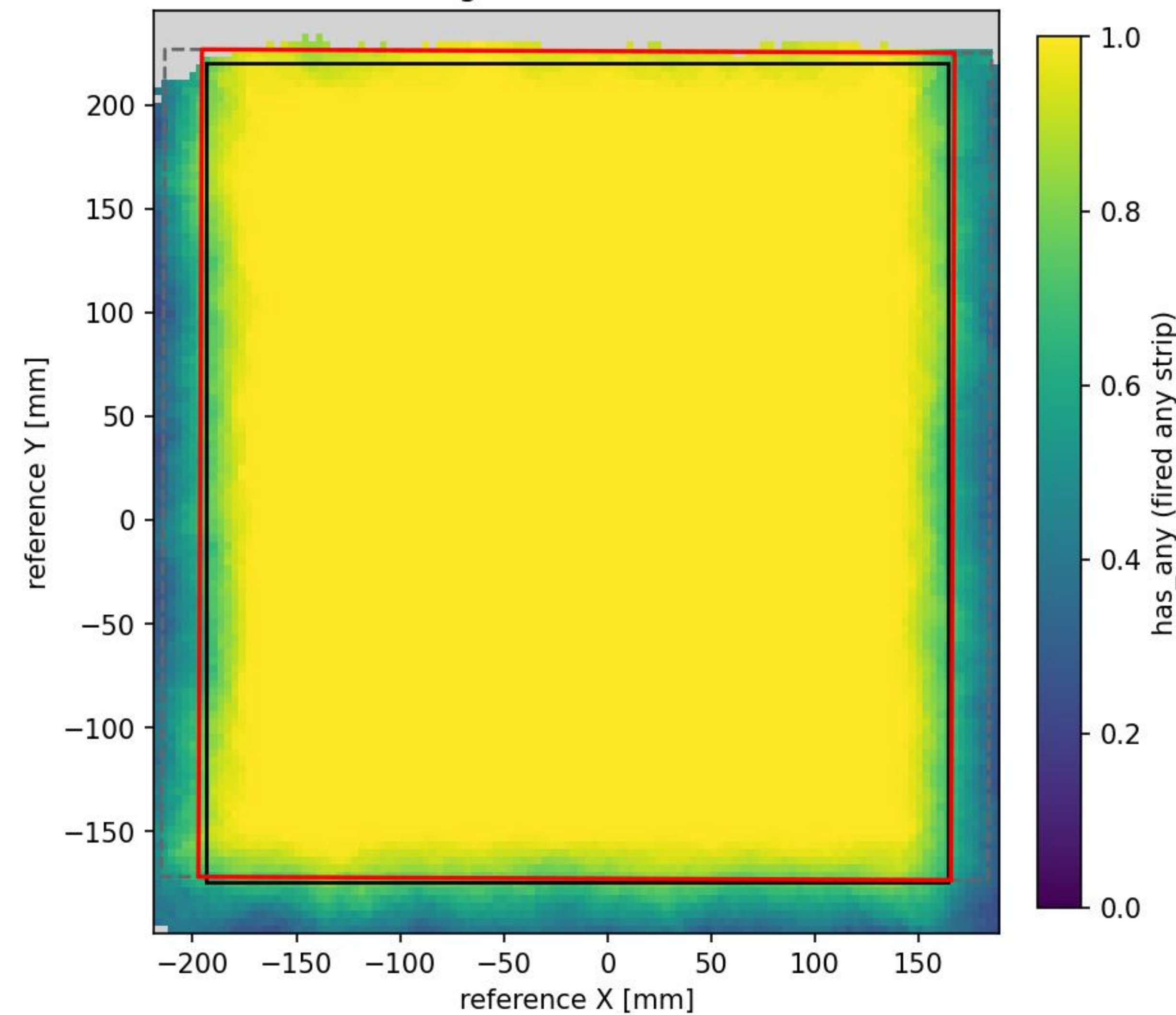
mx17_6 has_any (fired any strip) sliding kernel r=25.0 mm
