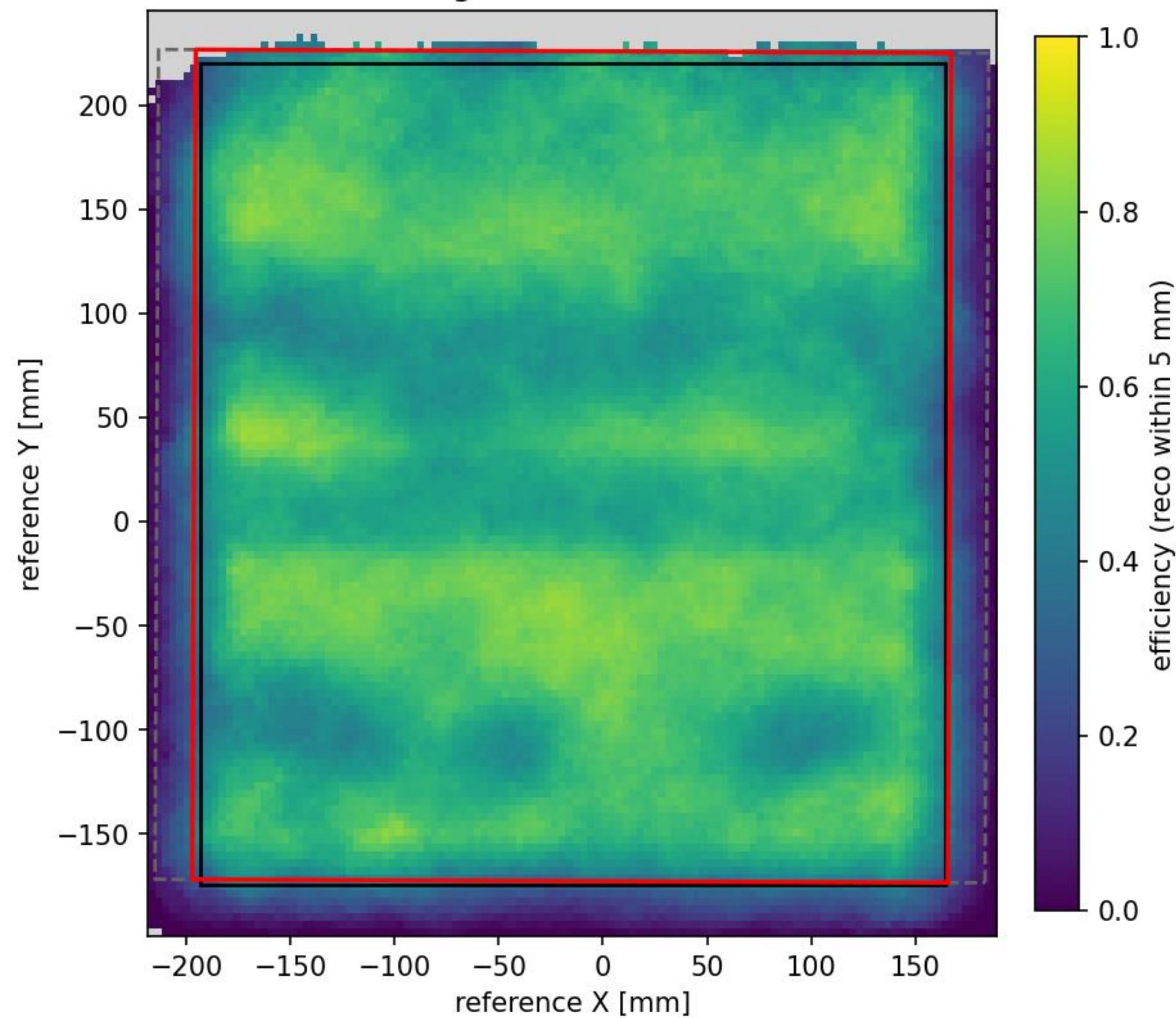
mx17_6 efficiency (reco within 5 mm) sliding kernel r=25.0 mm
