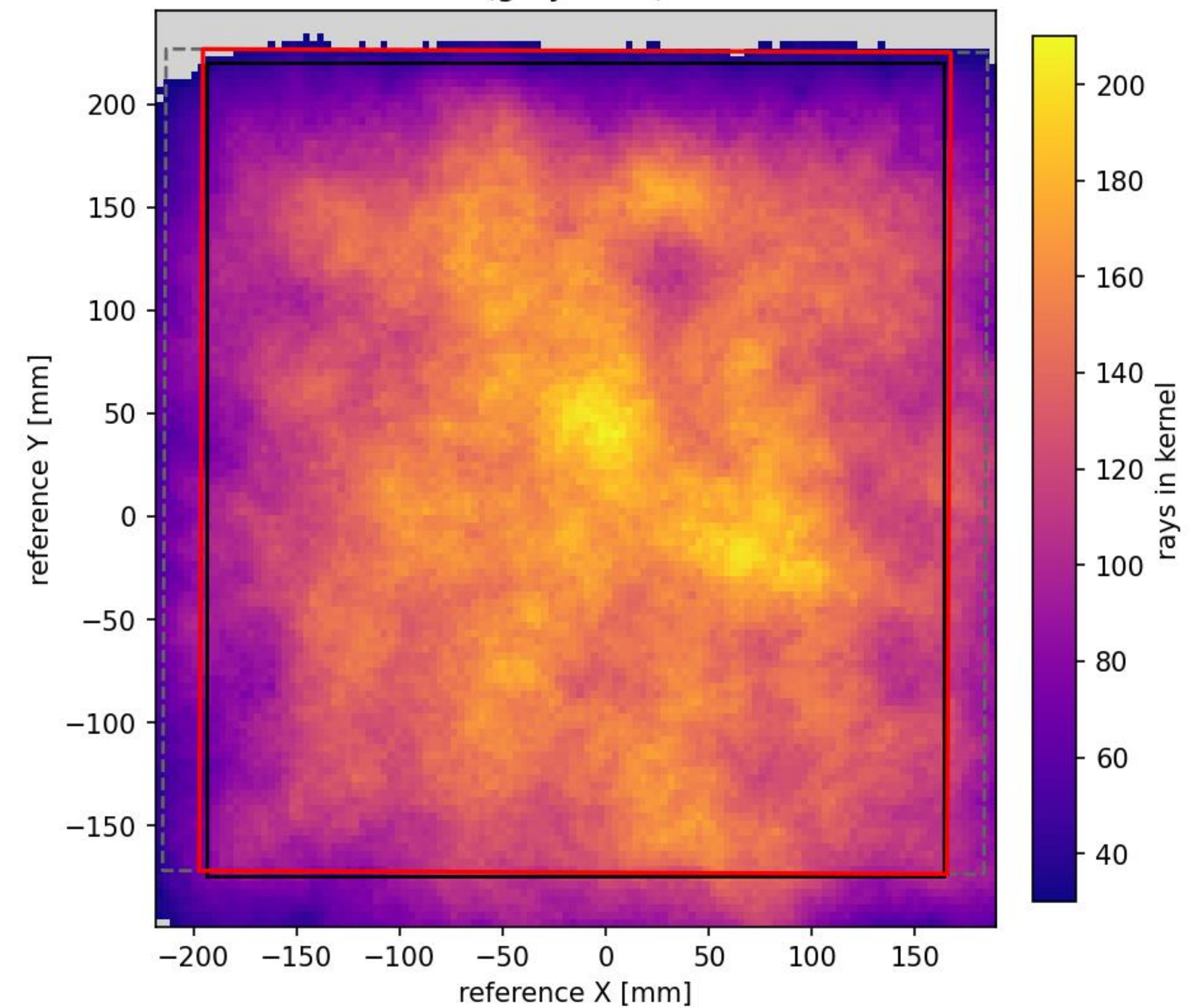
rays per kernel (grey < 30)
