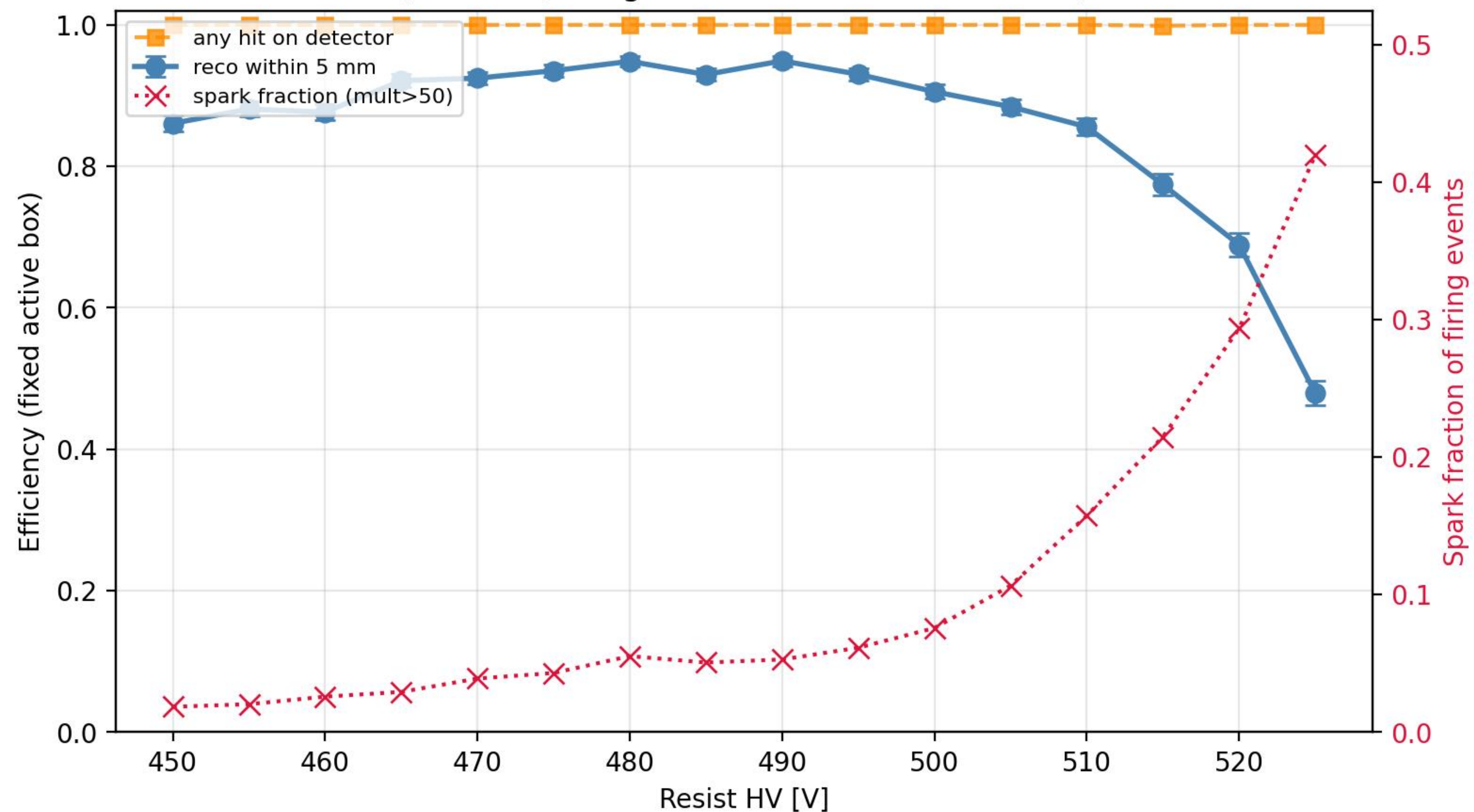
mx17_2 efficiency + spark rate vs resist HV — mx17_det2_det3_overnight_6-22-26 ( r < 5 mm; integrated over fixed active area)
