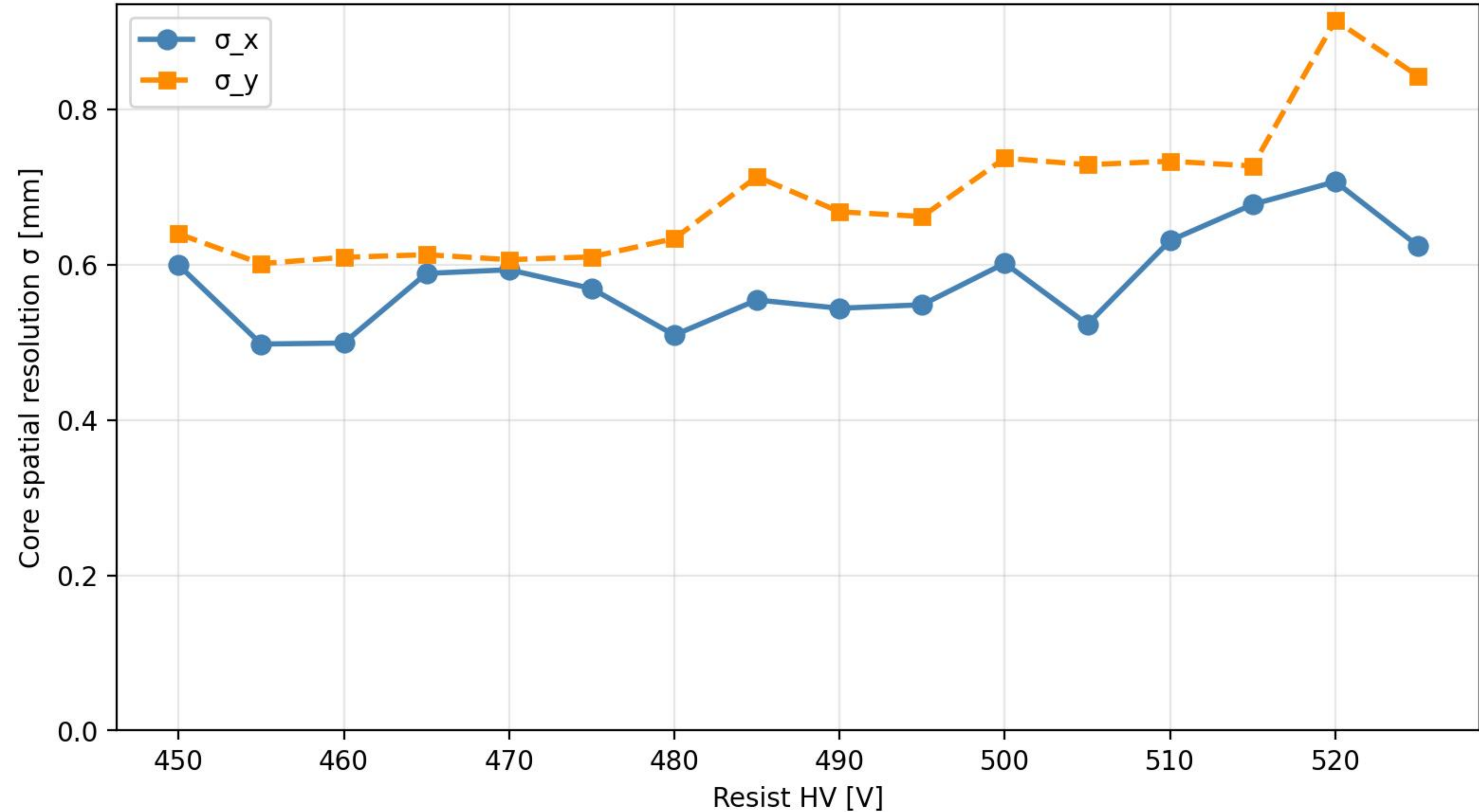
mx17_3 resolution vs resist HV — mx17_det2_det3_overnight_6-22-26 (Gaussian core of in-box residuals)
