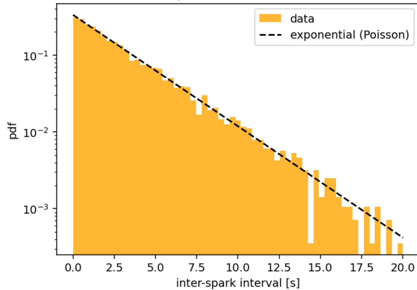
(b) inter-spark intervals match exponential \rightarrow random in time
