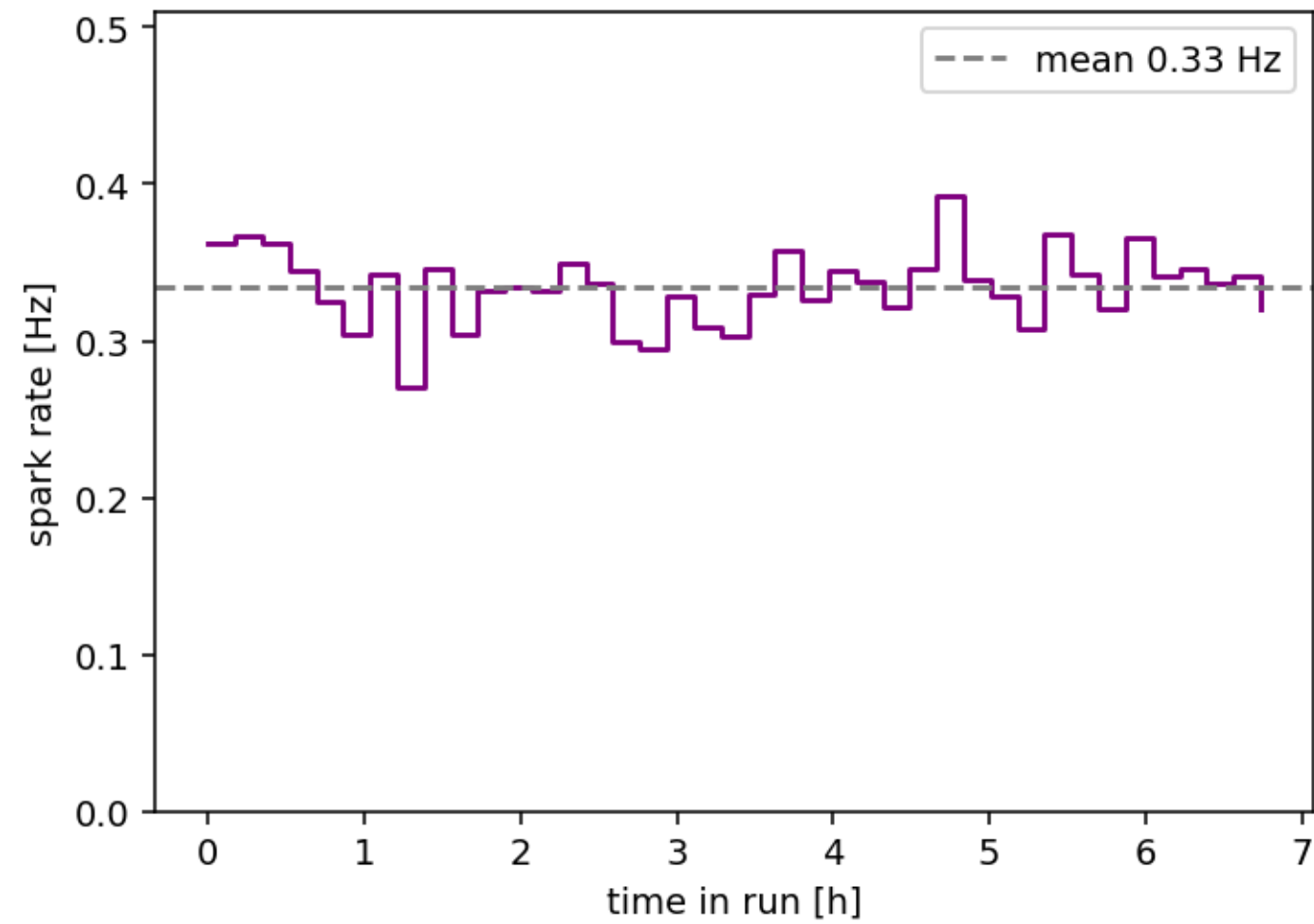
(a) spark rate vs time flat \rightarrow no HV bursts
