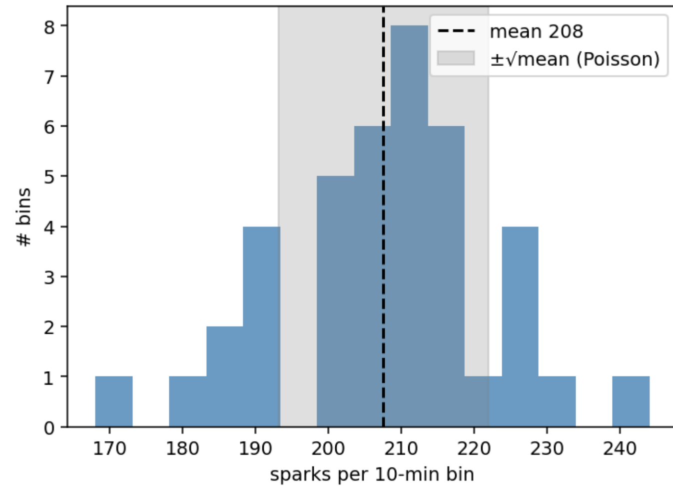
(c) counts/bin std=14 vs \sqrt{\text{mean}}=14 \rightarrow Poisson
