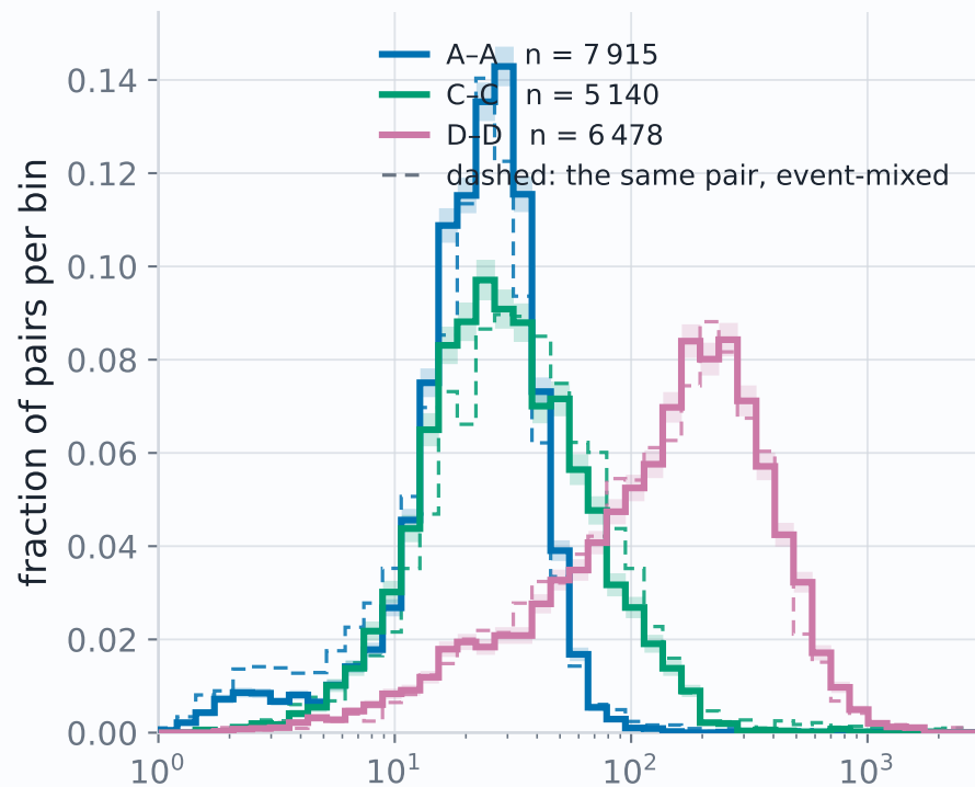
intra
