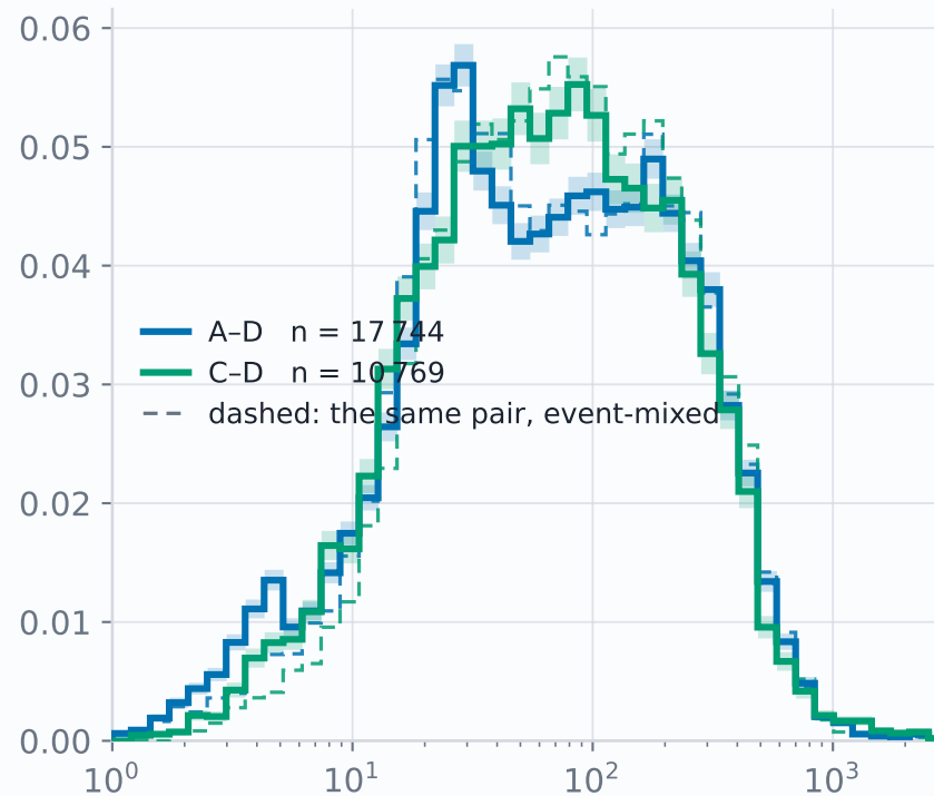
perpendicular
