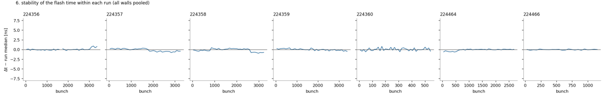
Figure 3: Within-run stability: pooling all 32 channels in 40 bins across a full three-hour run, the bin-to-bin spread is 0.25–0.39 ns and the maximum excursion 1.4 ns.
