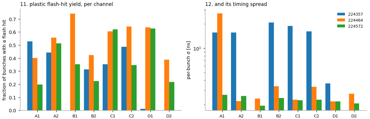
Figure 9: Per-channel flash-hit yield and timing spread for the eight plastic readouts in the three reference runs.
