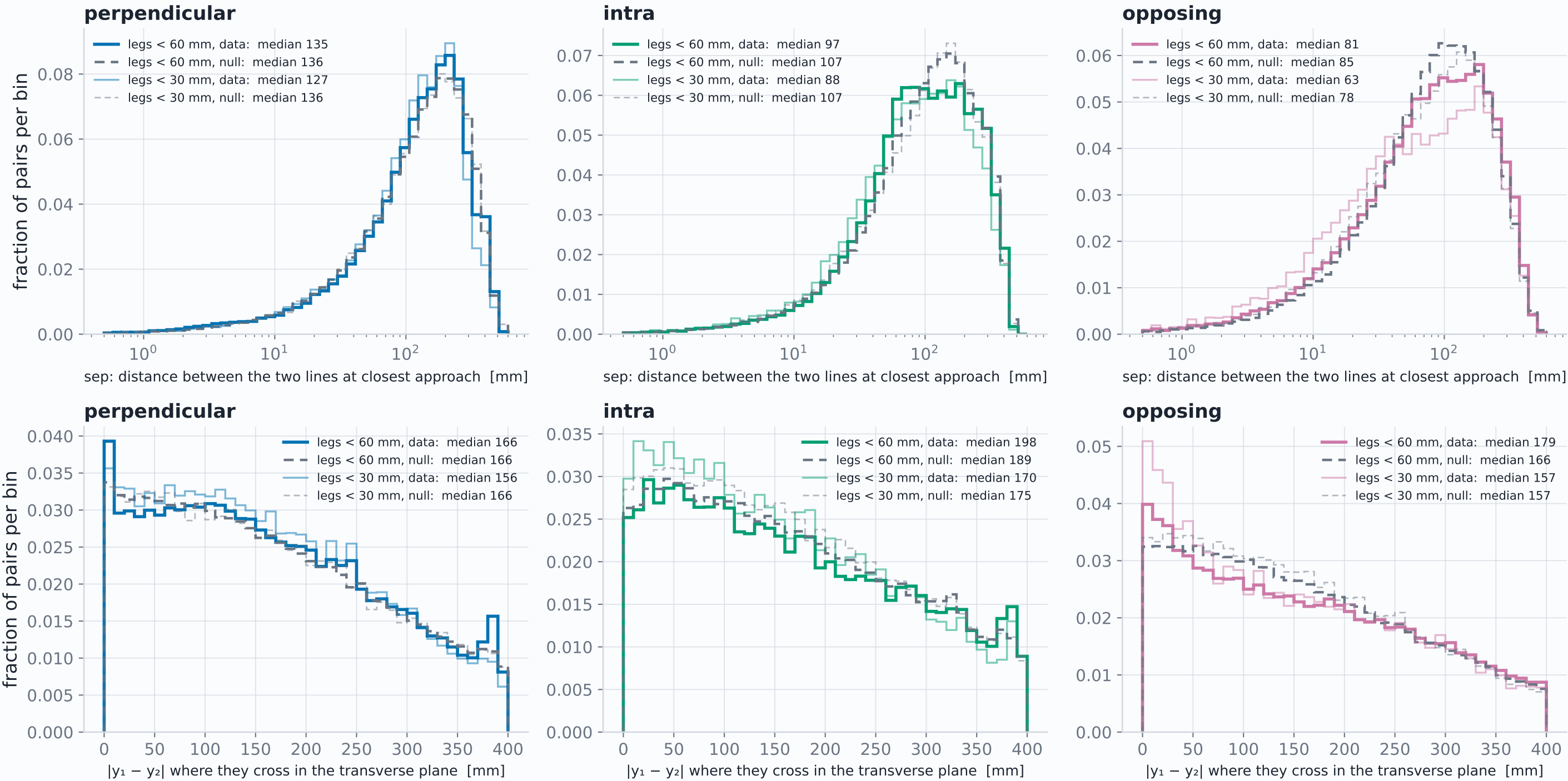
Top: the 3D distance of closest approach between the two fitted lines. Bottom: the y disagreement at their transverse crossing (the transverse separation there is zero by construction).
