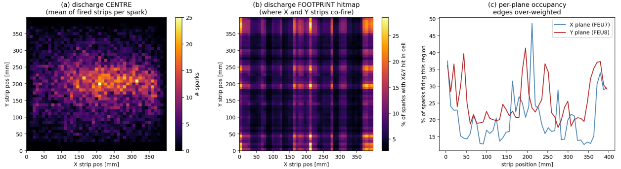
Figure 6: Spark hitmaps (detector strip frame). (a) discharge centre (mean of fired strips per spark); (b) footprint — % of sparks with X & Y activity per cell, a fixed edge+hot-strip grid; (c) per-plane occupancy, edges over-weighted.
