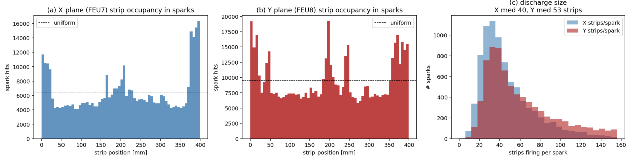
Figure 5: Where. (a,b) strip occupancy in sparks for the X and Y planes vs a uniform baseline — edge peaks (both planes) and fixed hot strips (Y); (c) strips firing per spark — Y discharges are larger than X.
