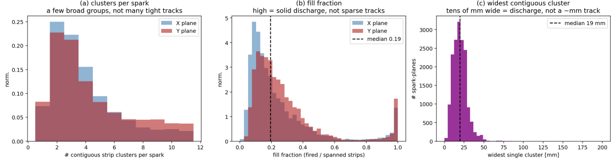
Figure 7: Detector-side shower check. (a) contiguous clusters per spark; (b) fill fraction; (c) widest contiguous cluster — median 19 mm, far wider than a \sim mm particle track, so the fired strips are discharge blobs, not tight tracks.
