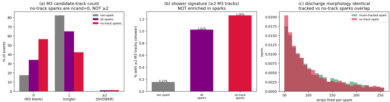
Figure 3: Shower test. (a) M3 candidate-track count by spark class — no-track sparks are \text{ncand} = 0/1 , not \geq 2 ; (b) the \geq 2 -track shower fraction is not meaningfully enriched in sparks; (c) muon-tracked and no-track sparks have identical discharge size (and span/duration/edge — see text).
