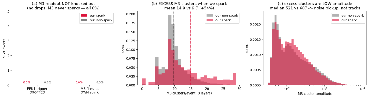
Figure 4: FEU1/M3 cross-talk. (a) M3 never drops a trigger nor fires its own spark on our sparks (both 0 %); (b) yet it records +54 % more clusters when we spark; (c) the excess clusters are low-amplitude — noise pickup, not tracks.
