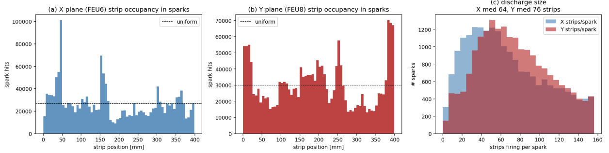
Figure 3: det7 locations: (a,b) edge peaks + hot strips in X and Y; (c) discharge size — larger than det3, Y harder than X.
