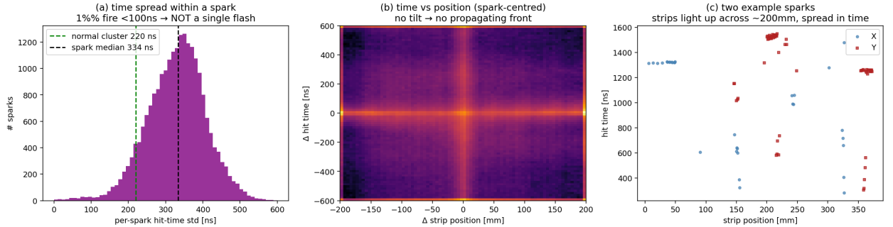
Figure 4: det7 time structure: (a) longer per-spark spread than det3; (b) no tilt (no propagating front); (c) example sparks across the whole plane, spread in time.
