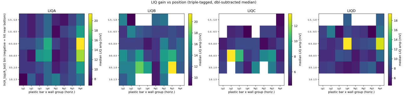
Figure 17: Median LIQ amplitude per position bin (triple-tagged, double sideband-subtracted). Columns: plastic bar \times wall group (left \rightarrow right as seen from the back); rows: vertical asymmetry bins (negative = hit near the bottom).
