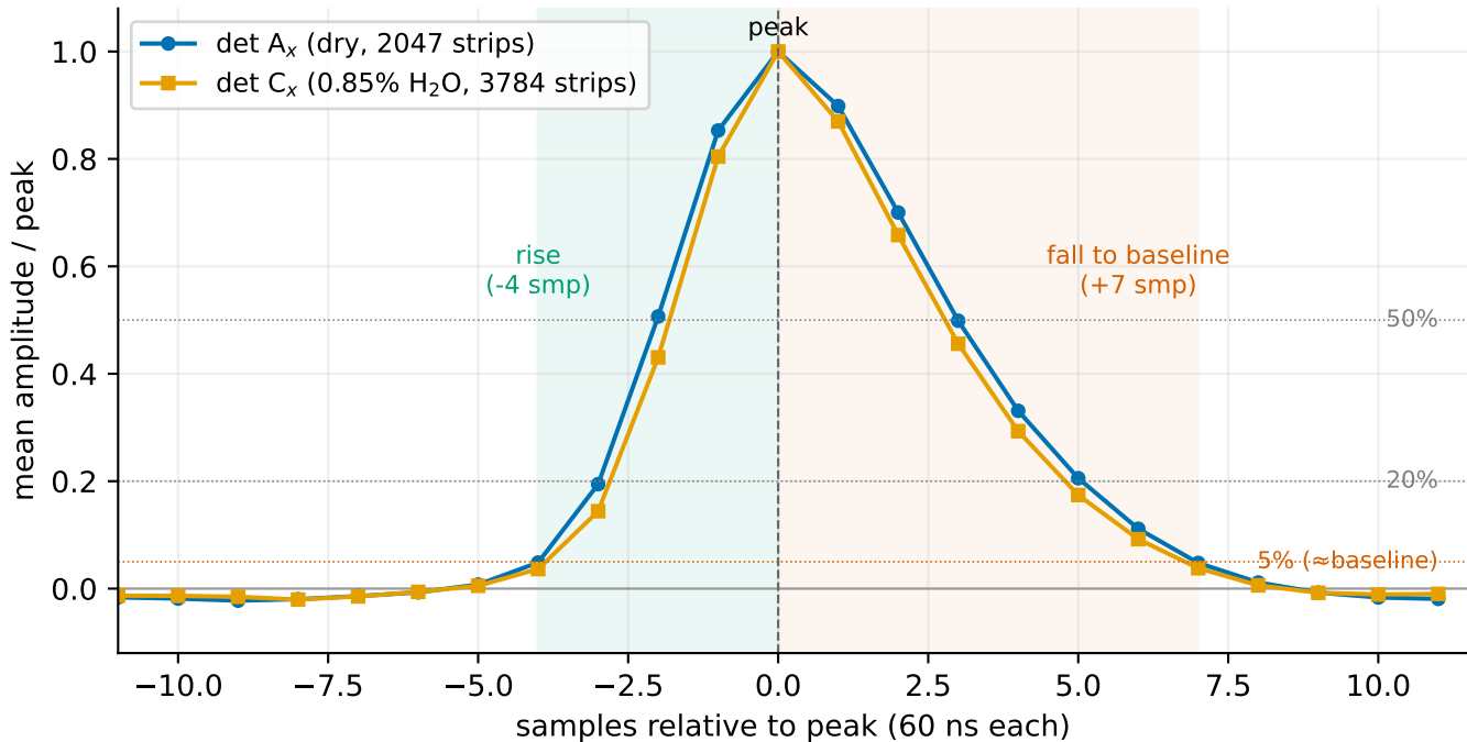
Measured DREAM pulse shape (cosmic hit strips): full footprint = peak-4 to peak+7
