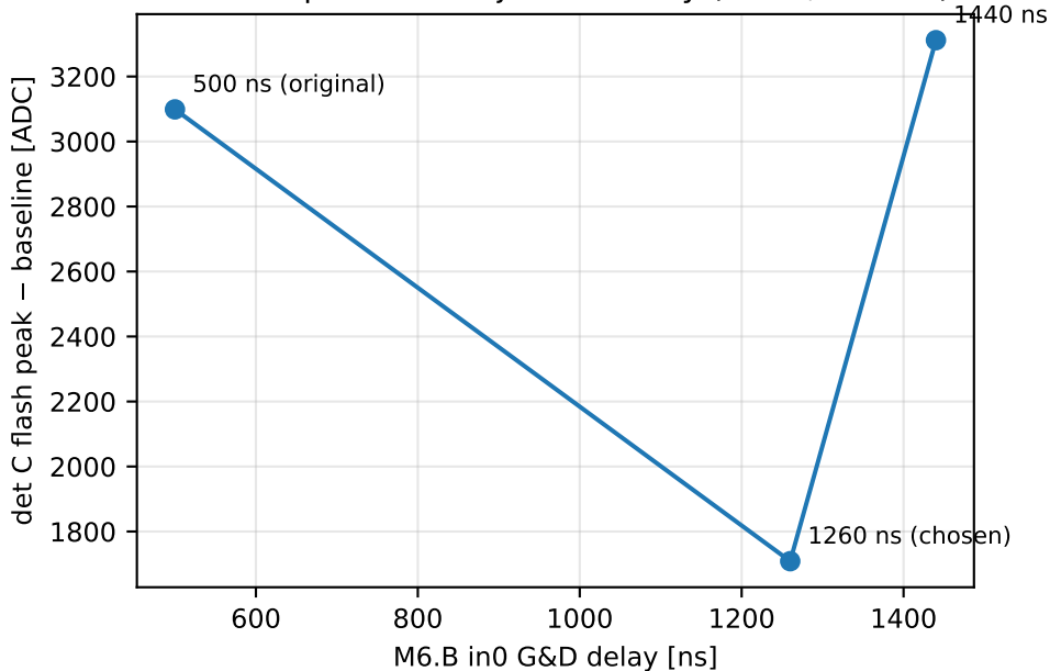
Flash amplitude vs injection delay (det C, FEU 07)
