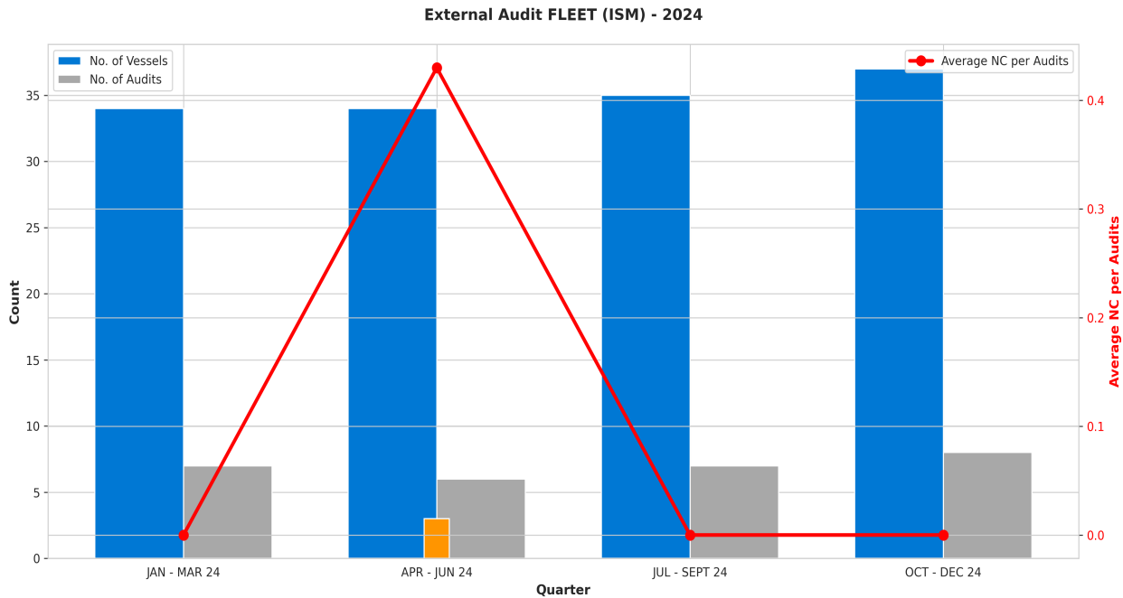
Chart 2: External Audit Fleet (ISM) - 2024 Quarterly
