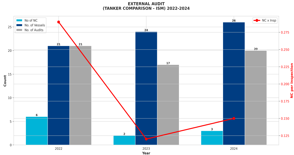
Chart 4: External Audit (Tanker Comparison - ISM) 2022-2024
