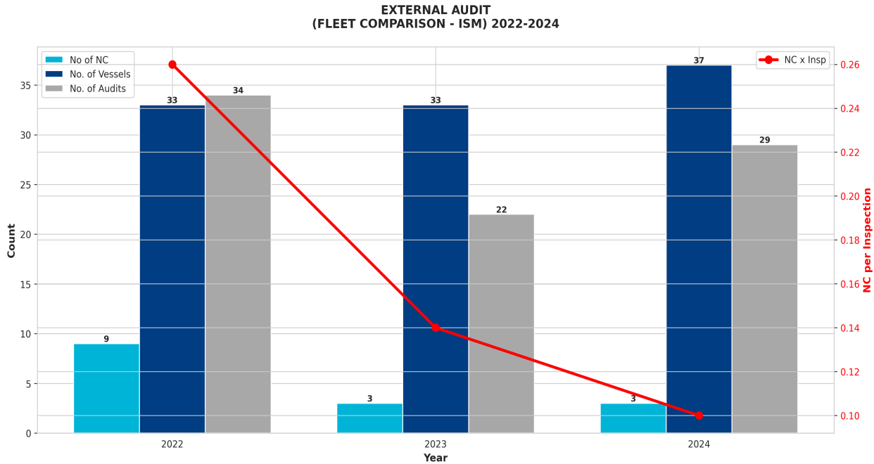
Chart 1: External Audit Fleet Comparison (2022-2024)
