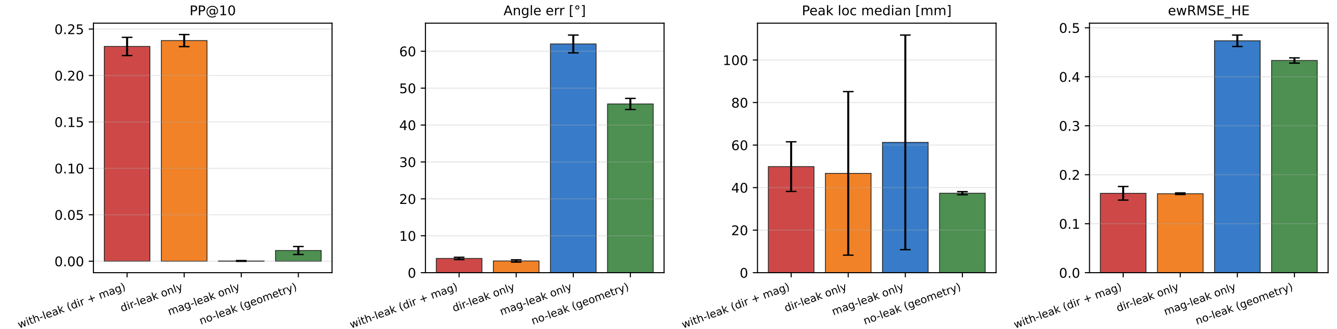
Leakage decomposition: identical model + training, swap x[:,3:6] (direction) and x[:,8] (magnitude)
