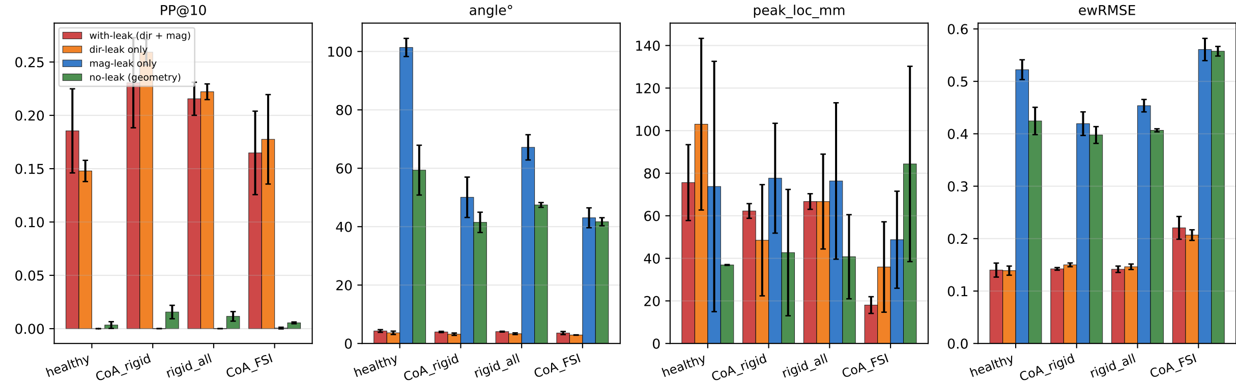
Per-pathology stratification (3-seed mean \pm std)
