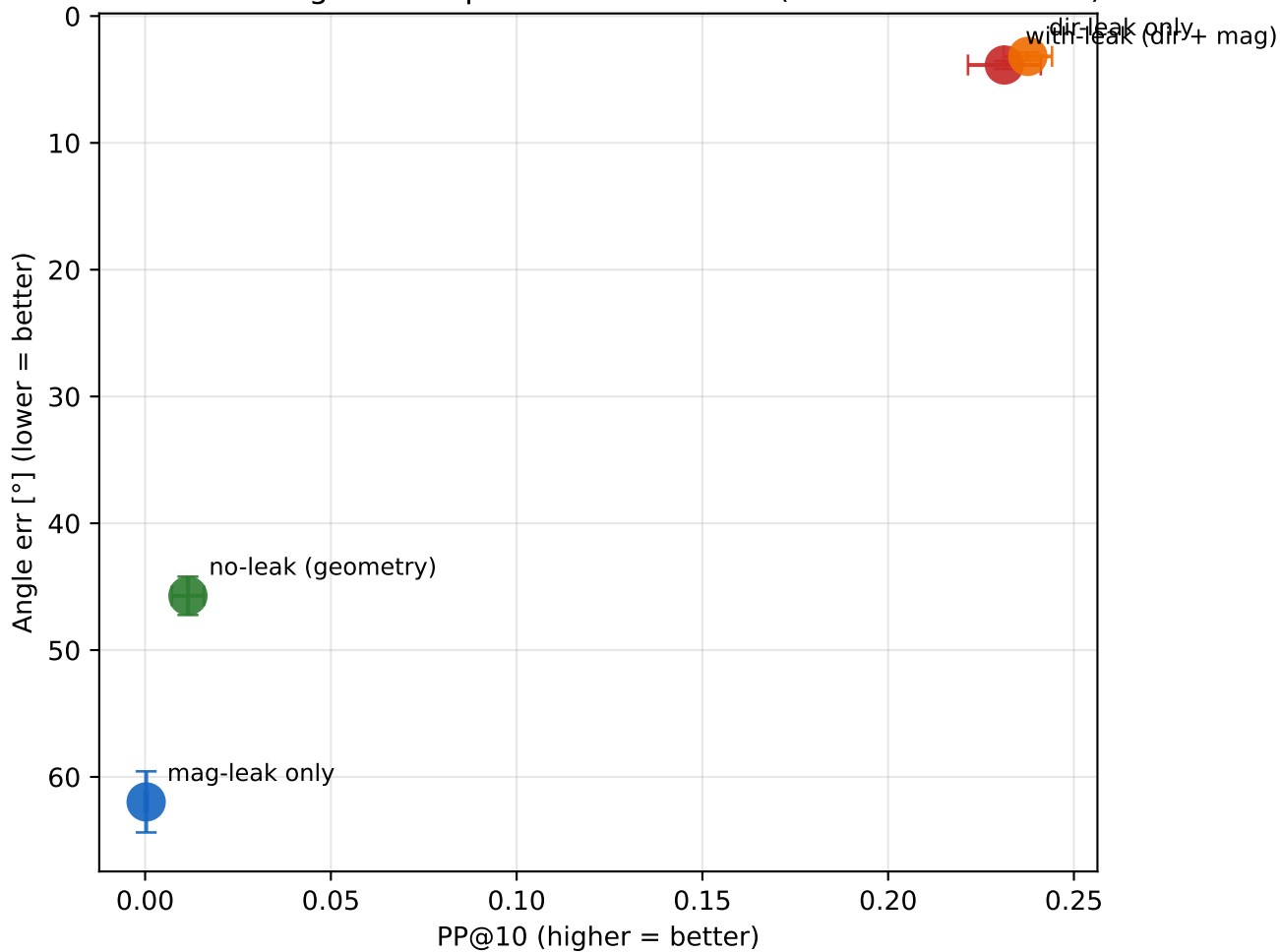
Feature-leakage decomposition on test set (3-seed mean \pm std)
