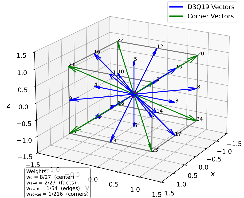
D3Q27 Lattice Model
