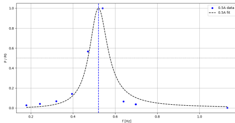
Figure 9: P/P_0(f) 0.5A
